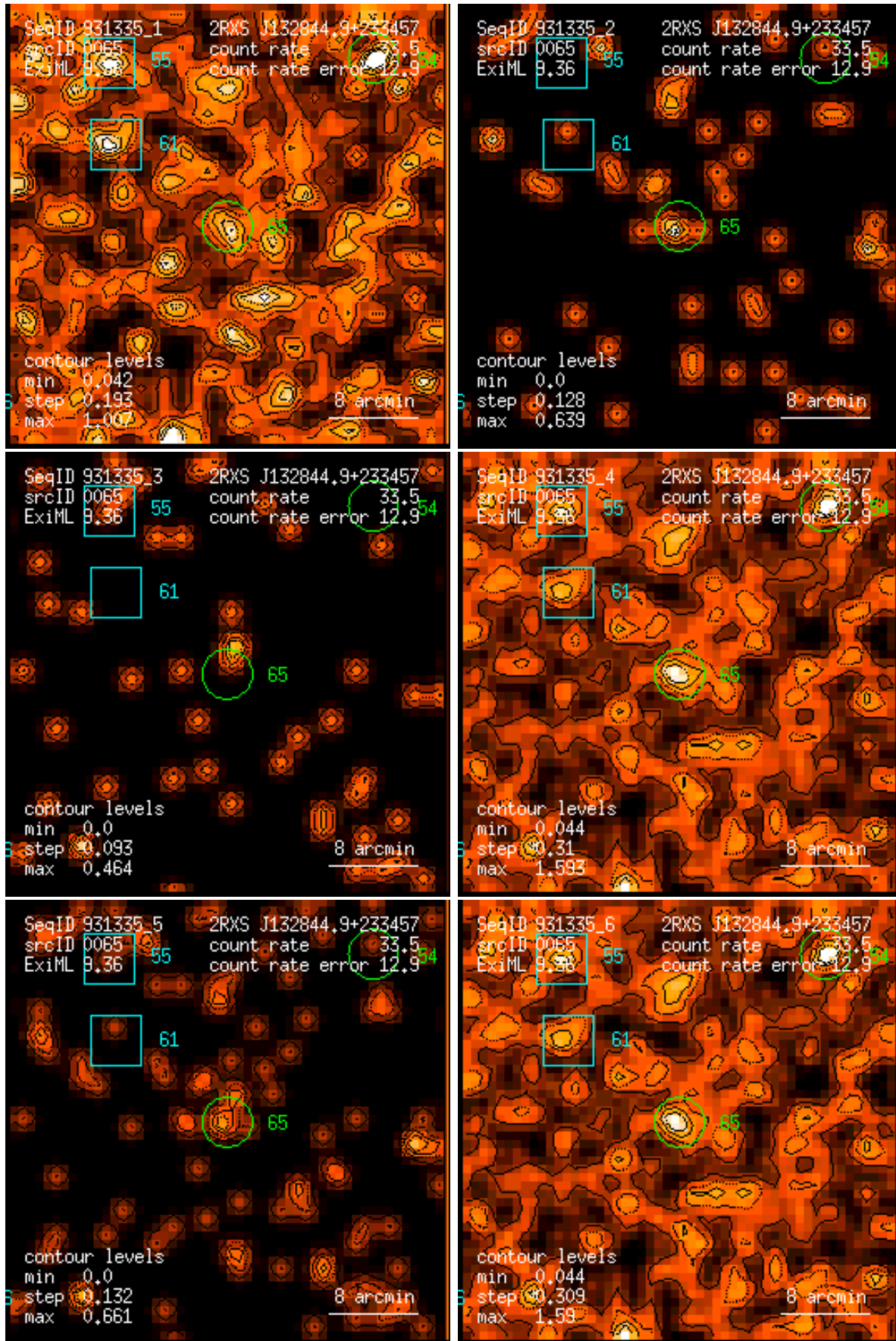
Figure 65: RASS 931335: detection 0065: band rate images, Gaussian filter: (1) PSPC channels 11 – 41, (2) 52 – 90, (3) 91 – 201, (4) 11 – 235, (5) 52 – 201, (6) 11 – 201. Broad band rates in counts/ks. Band rate contour levels in counts/ks/arcmin 2 .
