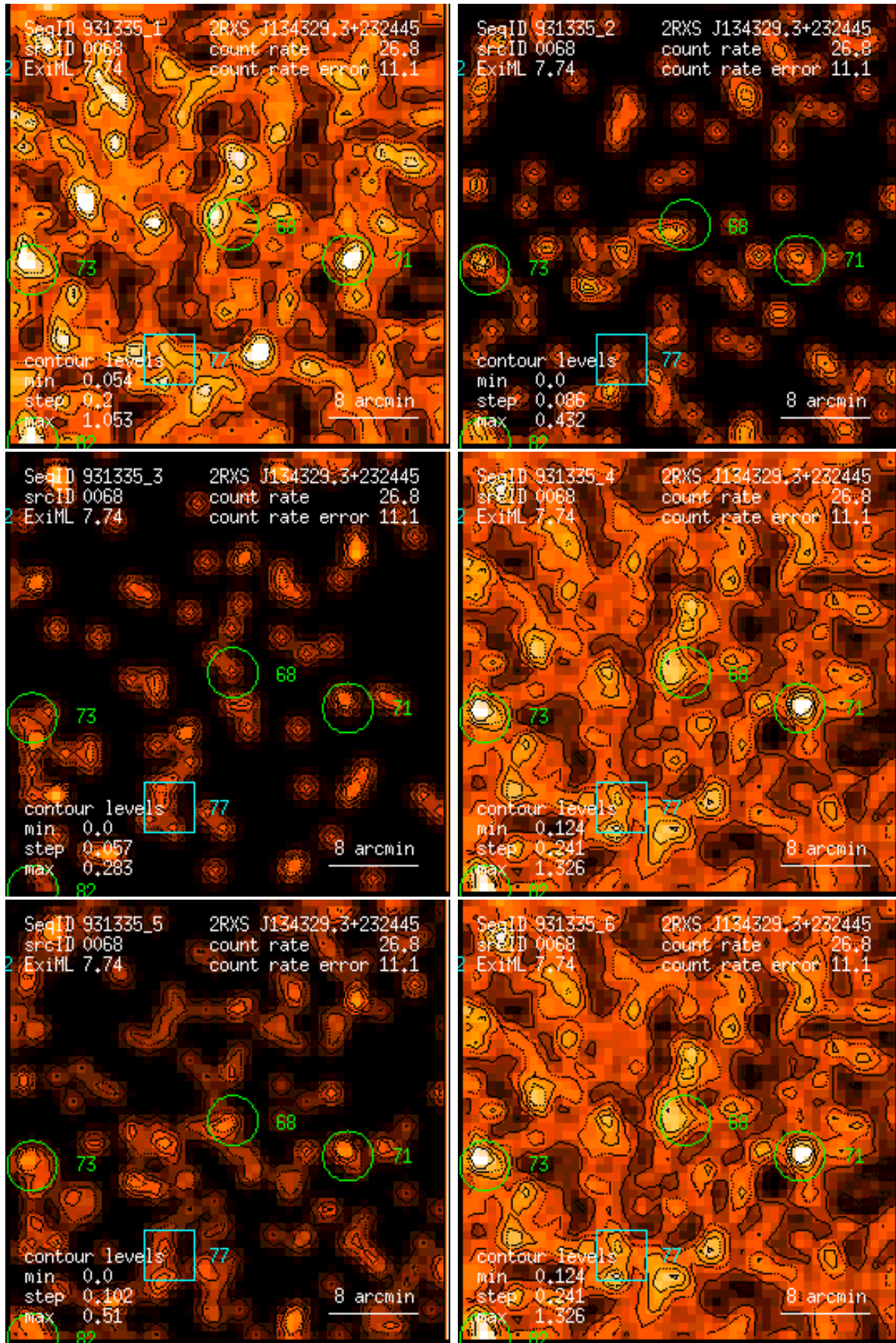
Figure 68: RASS 931335: detection 0068: band rate images, Gaussian filter: (1) PSPC channels 11 – 41, (2) 52 – 90, (3) 91 – 201, (4) 11 – 235, (5) 52 – 201, (6) 11 – 201. Broad band rates in counts/ks. Band rate contour levels in counts/ks/arcmin 2 .
