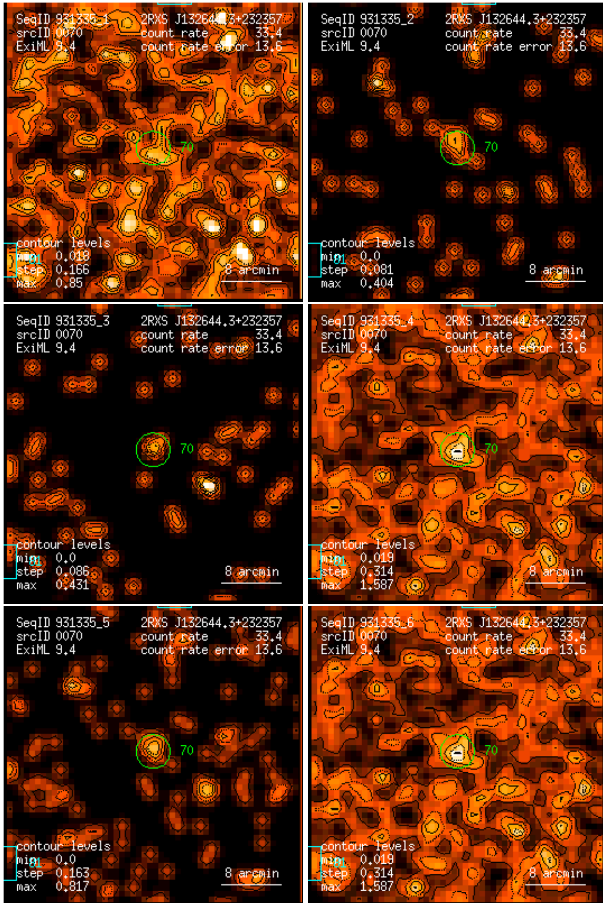
Figure 70: RASS 931335: detection 0070: band rate images, Gaussian filter: (1) PSPC channels 11 – 41, (2) 52 – 90, (3) 91 – 201, (4) 11 – 235, (5) 52 – 201, (6) 11 – 201. Broad band rates in counts/ks. Band rate contour levels in counts/ks/arcmin 2 .
