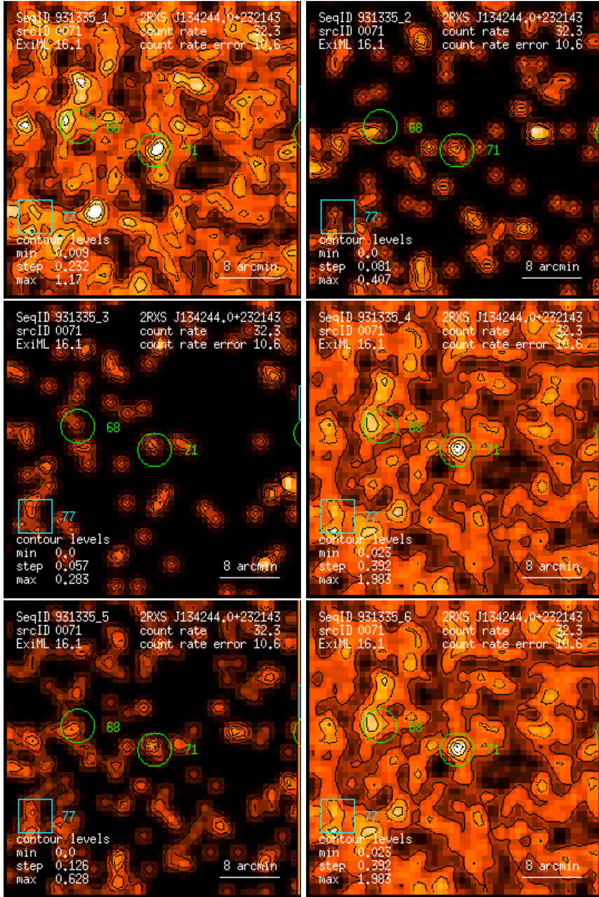
Figure 71: RASS 931335: detection 0071: band rate images, Gaussian filter: (1) PSPC channels 11 – 41, (2) 52 – 90, (3) 91 – 201, (4) 11 – 235, (5) 52 – 201, (6) 11 – 201. Broad band rates in counts/ks. Band rate contour levels in counts/ks/arcmin 2 .
