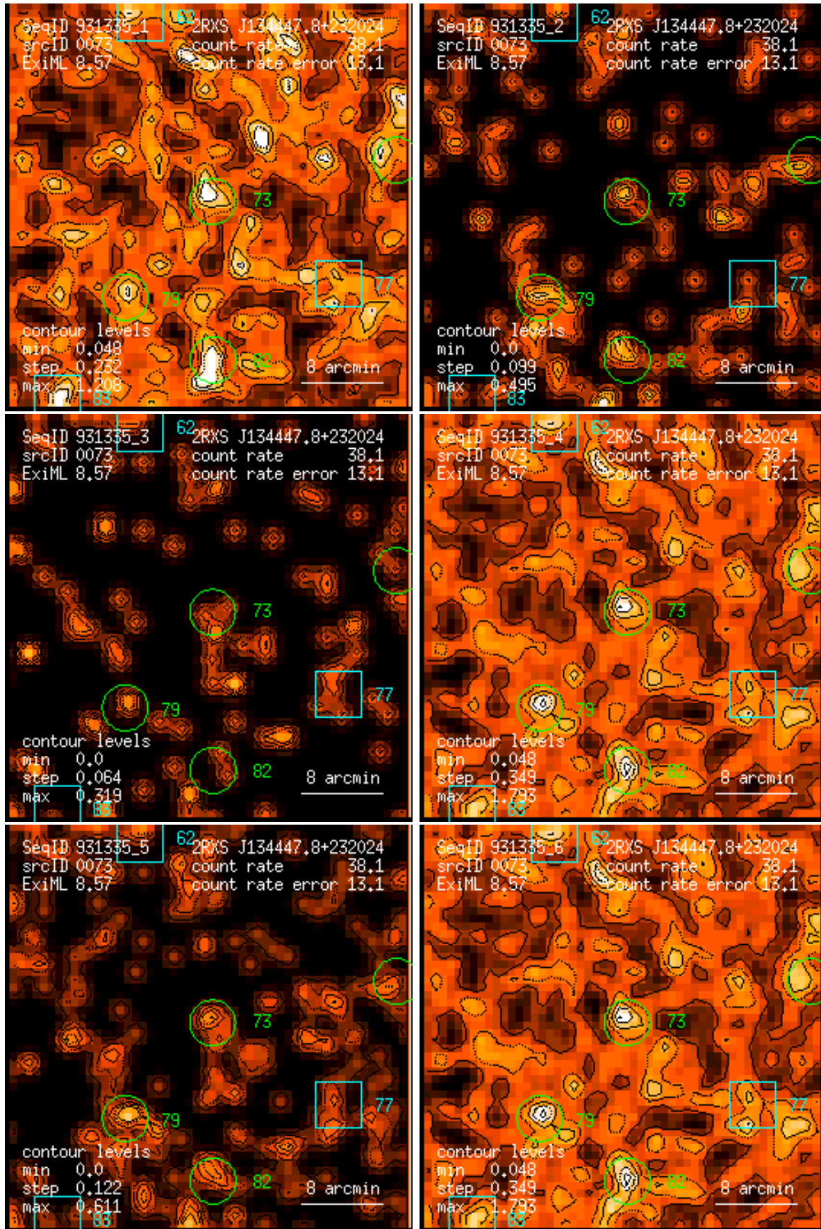
Figure 73: RASS 931335: detection 0073: band rate images, Gaussian filter: (1) PSPC channels 11 – 41, (2) 52 – 90, (3) 91 – 201, (4) 11 – 235, (5) 52 – 201, (6) 11 – 201. Broad band rates in counts/ks. Band rate contour levels in counts/ks/arcmin 2 .
