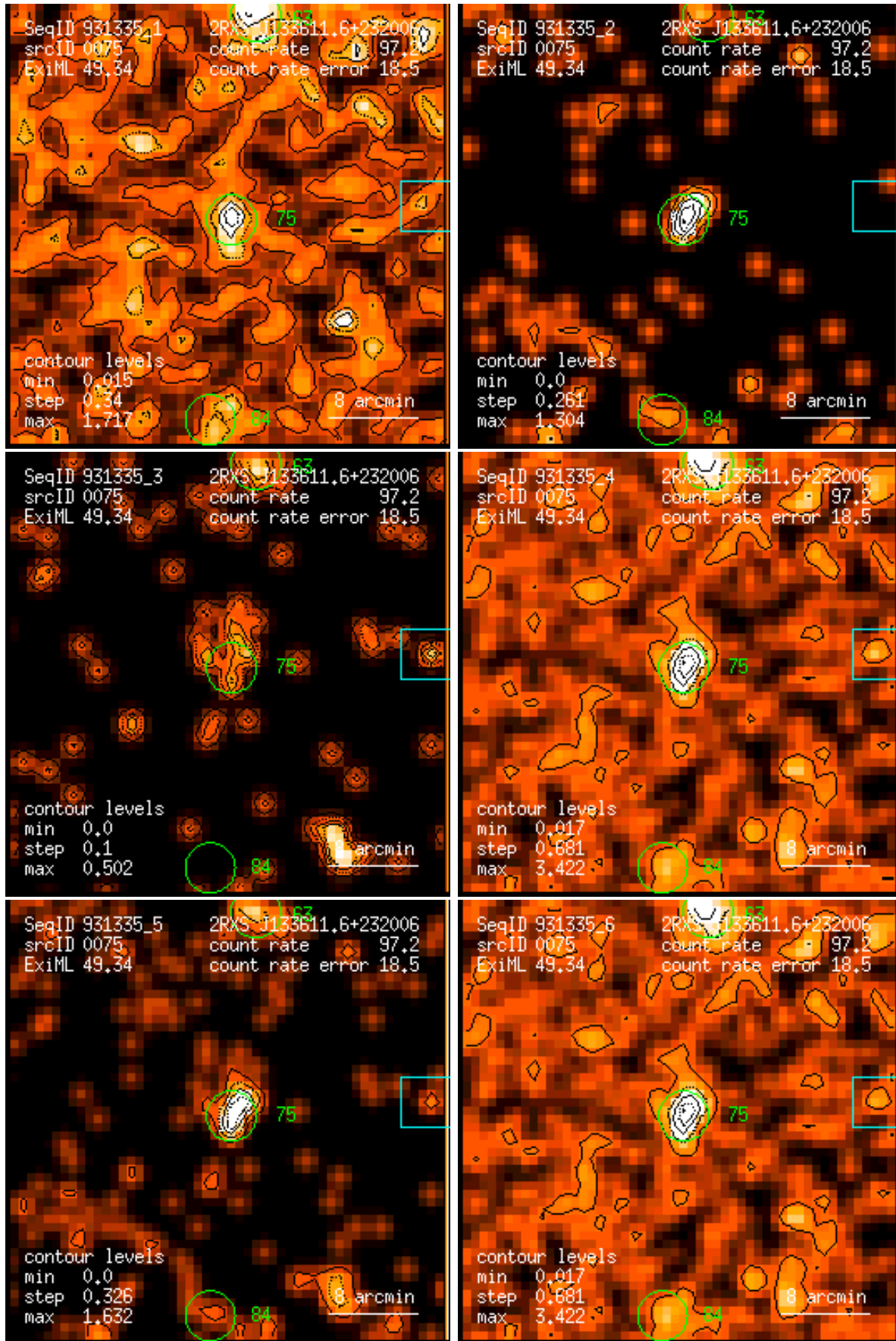
Figure 75: RASS 931335: detection 0075: band rate images, Gaussian filter: (1) PSPC channels 11 – 41, (2) 52 – 90, (3) 91 – 201, (4) 11 – 235, (5) 52 – 201, (6) 11 – 201. Broad band rates in counts/ks. Band rate contour levels in counts/ks/arcmin 2 .
