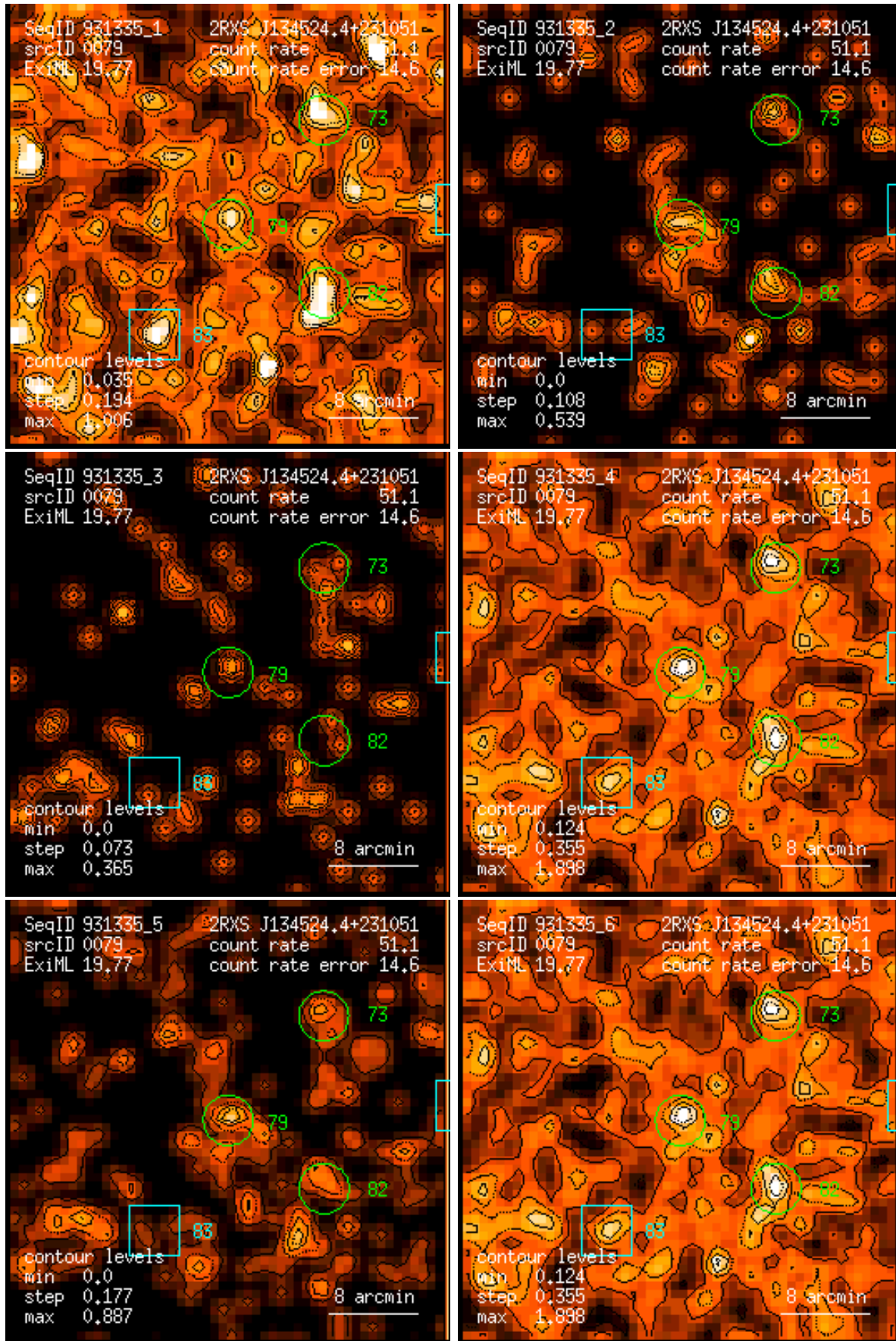
Figure 79: RASS 931335: detection 0079: band rate images, Gaussian filter: (1) PSPC channels 11 – 41, (2) 52 – 90, (3) 91 – 201, (4) 11 – 235, (5) 52 – 201, (6) 11 – 201. Broad band rates in counts/ks. Band rate contour levels in counts/ks/arcmin 2 .
