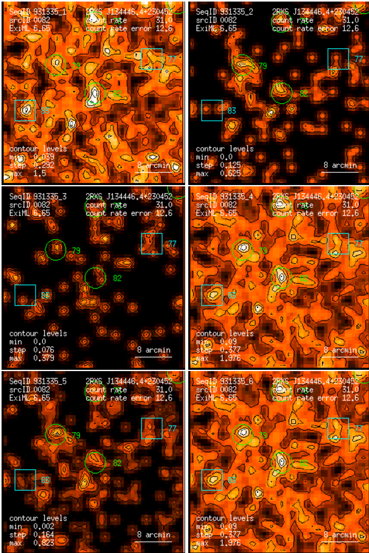
Figure 82: RASS 931335: detection 0082: band rate images, Gaussian filter: (1) PSPC channels 11 – 41, (2) 52 – 90, (3) 91 – 201, (4) 11 – 235, (5) 52 – 201, (6) 11 – 201. Broad band rates in counts/ks. Band rate contour levels in counts/ks/arcmin 2 .
