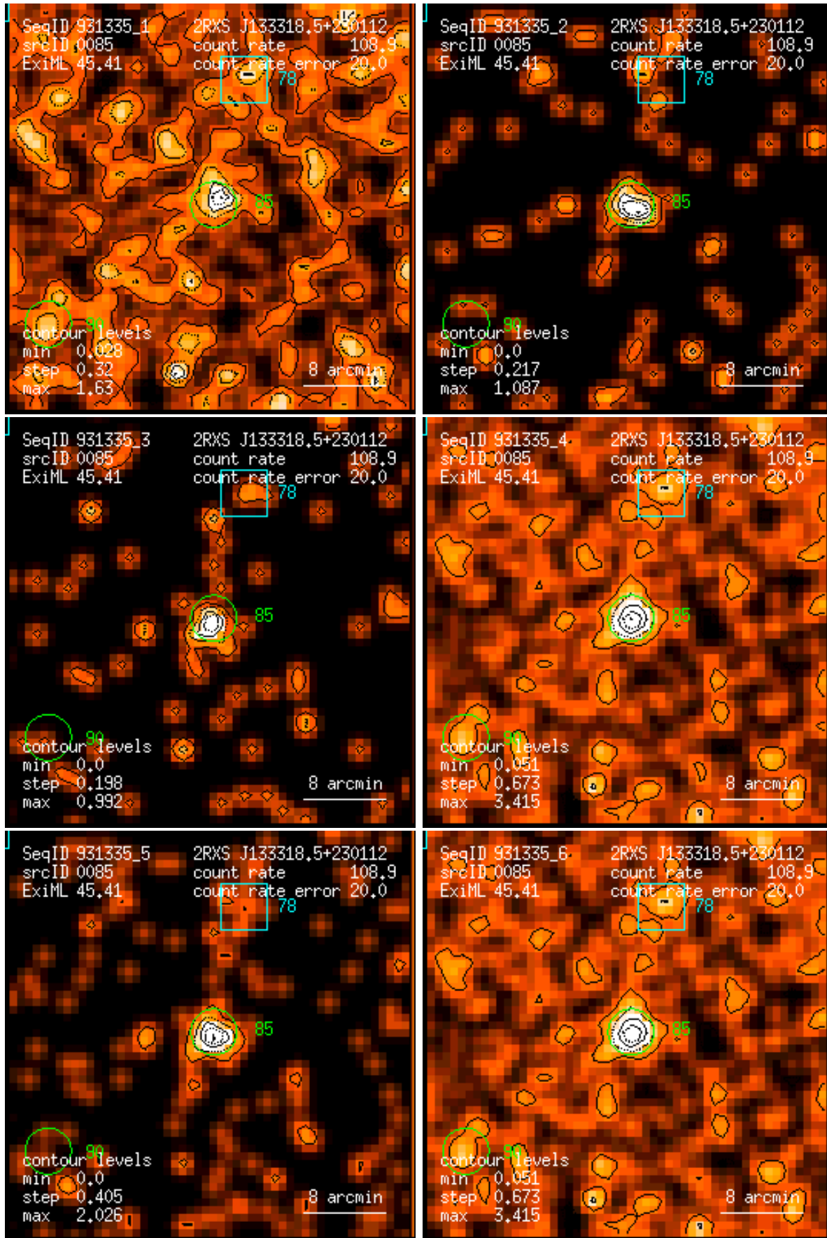
Figure 85: RASS 931335: detection 0085: band rate images, Gaussian filter: (1) PSPC channels 11 – 41, (2) 52 – 90, (3) 91 – 201, (4) 11 – 235, (5) 52 – 201, (6) 11 – 201. Broad band rates in counts/ks. Band rate contour levels in counts/ks/arcmin 2 .
