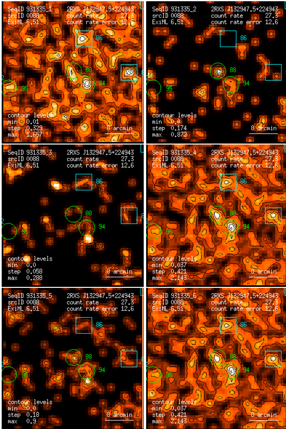
Figure 88: RASS 931335: detection 0088: band rate images, Gaussian filter: (1) PSPC channels 11 – 41, (2) 52 – 90, (3) 91 – 201, (4) 11 – 235, (5) 52 – 201, (6) 11 – 201. Broad band rates in counts/ks. Band rate contour levels in counts/ks/arcmin 2 .
