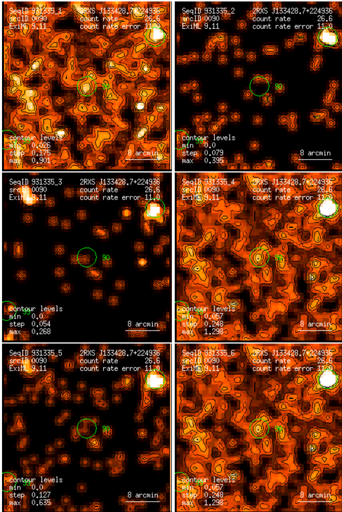
Figure 90: RASS 931335: detection 0090: band rate images, Gaussian filter: (1) PSPC channels 11 – 41, (2) 52 – 90, (3) 91 – 201, (4) 11 – 235, (5) 52 – 201, (6) 11 – 201. Broad band rates in counts/ks. Band rate contour levels in counts/ks/arcmin 2 .
