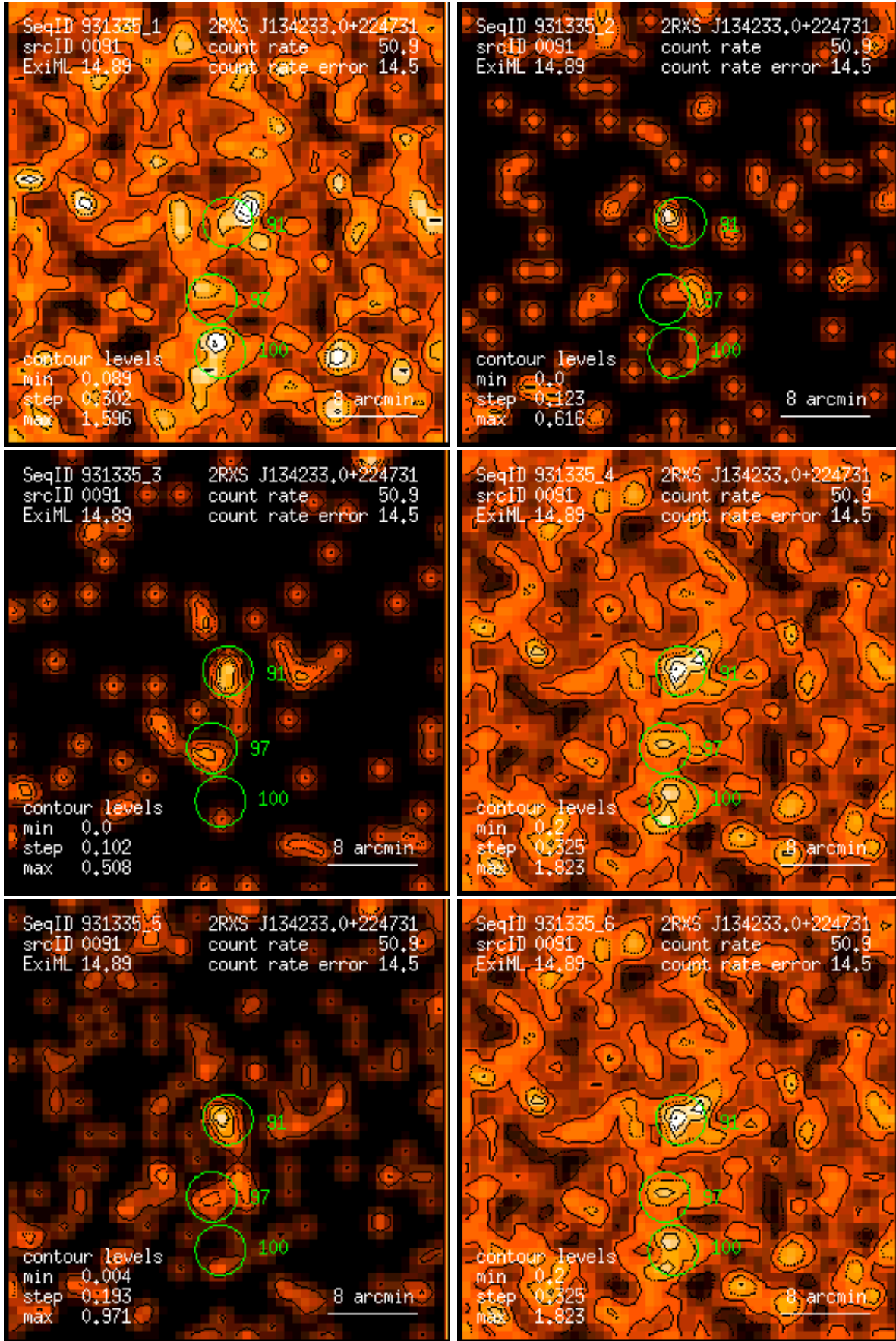
Figure 91: RASS 931335: detection 0091: band rate images, Gaussian filter: (1) PSPC channels 11 – 41, (2) 52 – 90, (3) 91 – 201, (4) 11 – 235, (5) 52 – 201, (6) 11 – 201. Broad band rates in counts/ks. Band rate contour levels in counts/ks/arcmin 2 .
