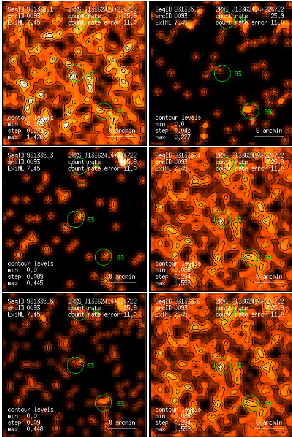
Figure 93: RASS 931335: detection 0093: band rate images, Gaussian filter: (1) PSPC channels 11 – 41, (2) 52 – 90, (3) 91 – 201, (4) 11 – 235, (5) 52 – 201, (6) 11 – 201. Broad band rates in counts/ks. Band rate contour levels in counts/ks/arcmin 2 .
