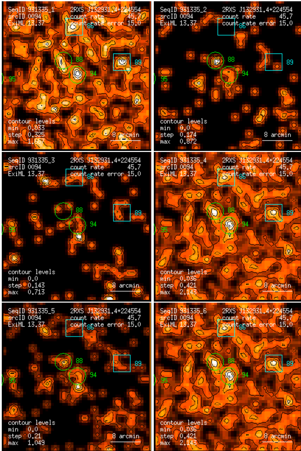
Figure 94: RASS 931335: detection 0094: band rate images, Gaussian filter: (1) PSPC channels 11 – 41, (2) 52 – 90, (3) 91 – 201, (4) 11 – 235, (5) 52 – 201, (6) 11 – 201. Broad band rates in counts/ks. Band rate contour levels in counts/ks/arcmin 2 .
