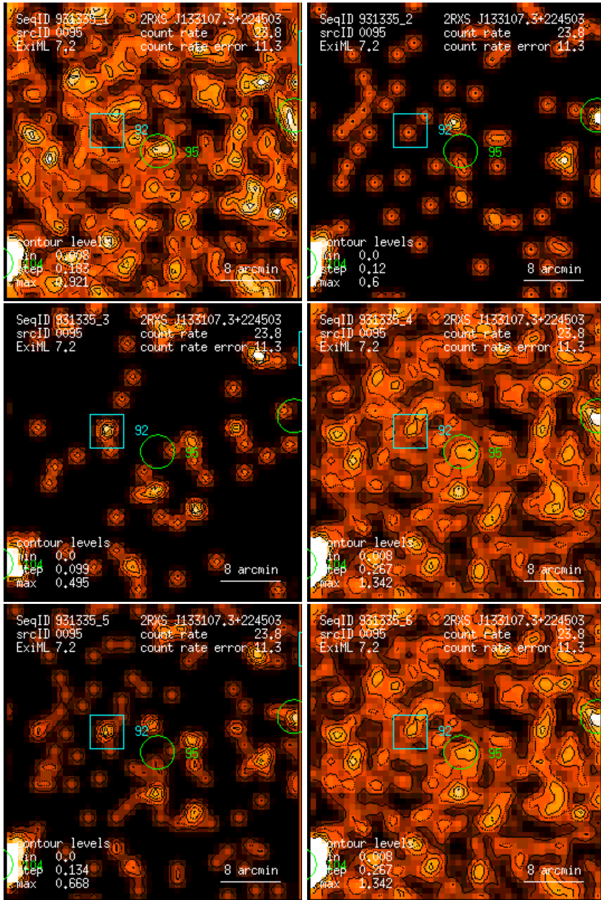
Figure 95: RASS 931335: detection 0095: band rate images, Gaussian filter: (1) PSPC channels 11 – 41, (2) 52 – 90, (3) 91 – 201, (4) 11 – 235, (5) 52 – 201, (6) 11 – 201. Broad band rates in counts/ks. Band rate contour levels in counts/ks/arcmin 2 .
