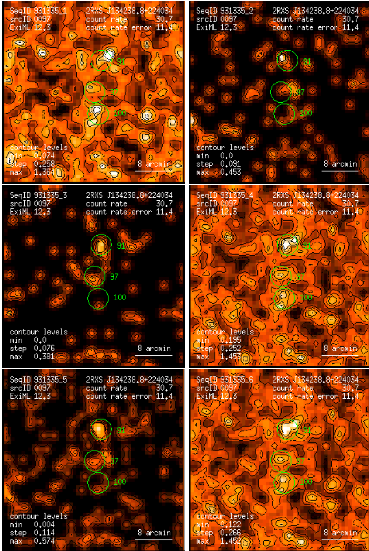
Figure 97: RASS 931335: detection 0097: band rate images, Gaussian filter: (1) PSPC channels 11 – 41, (2) 52 – 90, (3) 91 – 201, (4) 11 – 235, (5) 52 – 201, (6) 11 – 201. Broad band rates in counts/ks. Band rate contour levels in counts/ks/arcmin 2 .
