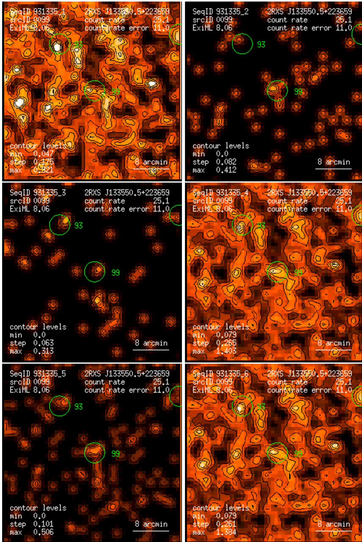
Figure 99: RASS 931335: detection 0099: band rate images, Gaussian filter: (1) PSPC channels 11 – 41, (2) 52 – 90, (3) 91 – 201, (4) 11 – 235, (5) 52 – 201, (6) 11 – 201. Broad band rates in counts/ks. Band rate contour levels in counts/ks/arcmin 2 .
