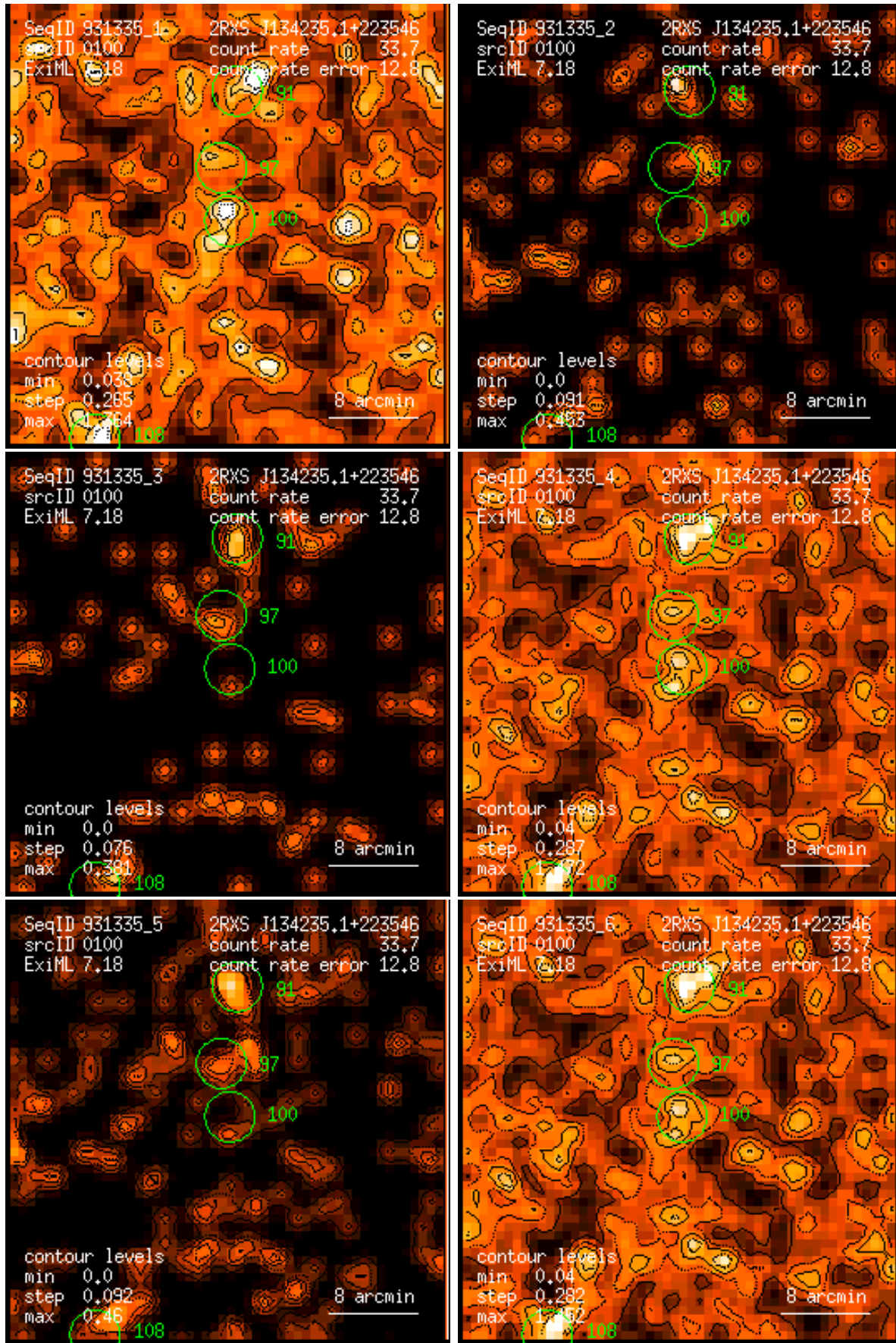
Figure 100: RASS 931335: detection 0100: band rate images, Gaussian filter: (1) PSPC channels 11 – 41, (2) 52 – 90, (3) 91 – 201, (4) 11 – 235, (5) 52 – 201, (6) 11 – 201. Broad band rates in counts/ks. Band rate contour levels in counts/ks/arcmin 2 .
