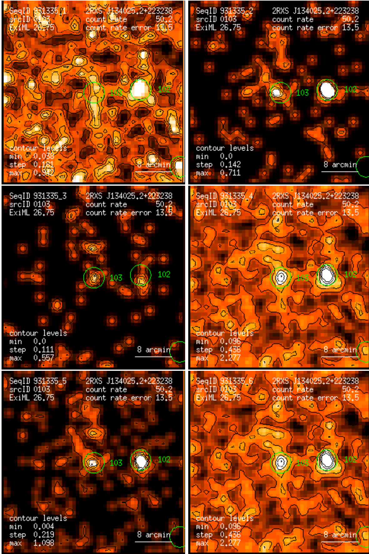
Figure 103: RASS 931335: detection 0103: band rate images, Gaussian filter: (1) PSPC channels 11 – 41, (2) 52 – 90, (3) 91 – 201, (4) 11 – 235, (5) 52 – 201, (6) 11 – 201. Broad band rates in counts/ks. Band rate contour levels in counts/ks/arcmin 2 .
