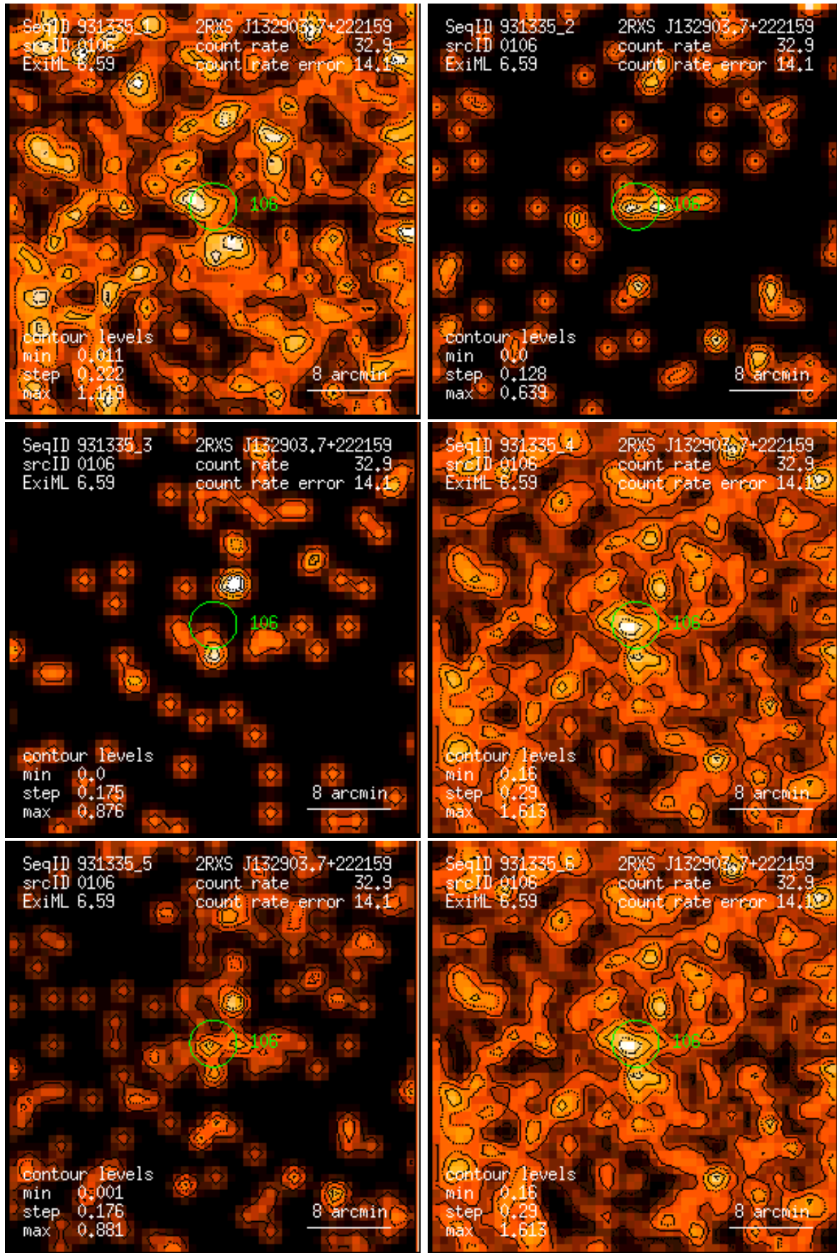
Figure 106: RASS 931335: detection 0106: band rate images, Gaussian filter: (1) PSPC channels 11 – 41, (2) 52 – 90, (3) 91 – 201, (4) 11 – 235, (5) 52 – 201, (6) 11 – 201. Broad band rates in counts/ks. Band rate contour levels in counts/ks/arcmin 2 .
