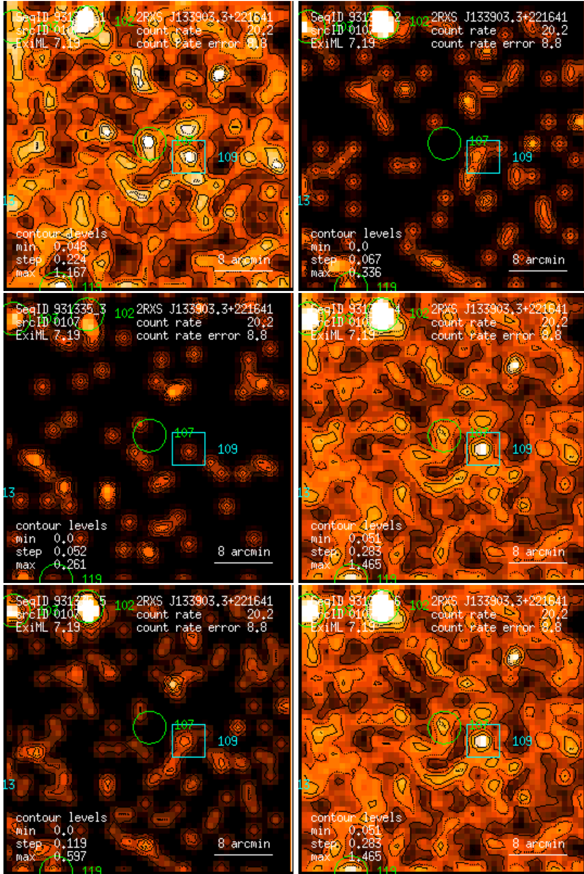
Figure 107: RASS 931335: detection 0107: band rate images, Gaussian filter: (1) PSPC channels 11 – 41, (2) 52 – 90, (3) 91 – 201, (4) 11 – 235, (5) 52 – 201, (6) 11 – 201. Broad band rates in counts/ks. Band rate contour levels in counts/ks/arcmin 2 .
