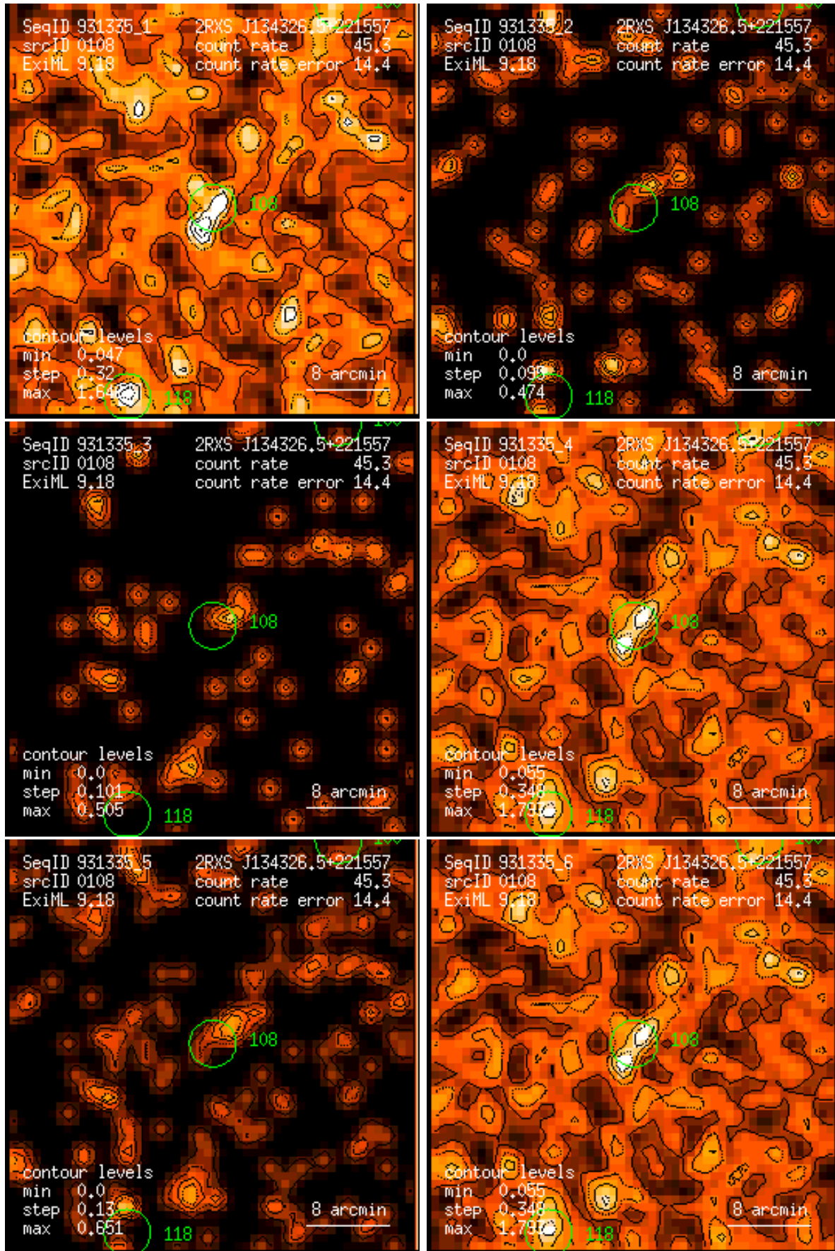
Figure 108: RASS 931335: detection 0108: band rate images, Gaussian filter: (1) PSPC channels 11 – 41, (2) 52 – 90, (3) 91 – 201, (4) 11 – 235, (5) 52 – 201, (6) 11 – 201. Broad band rates in counts/ks. Band rate contour levels in counts/ks/arcmin 2 .
