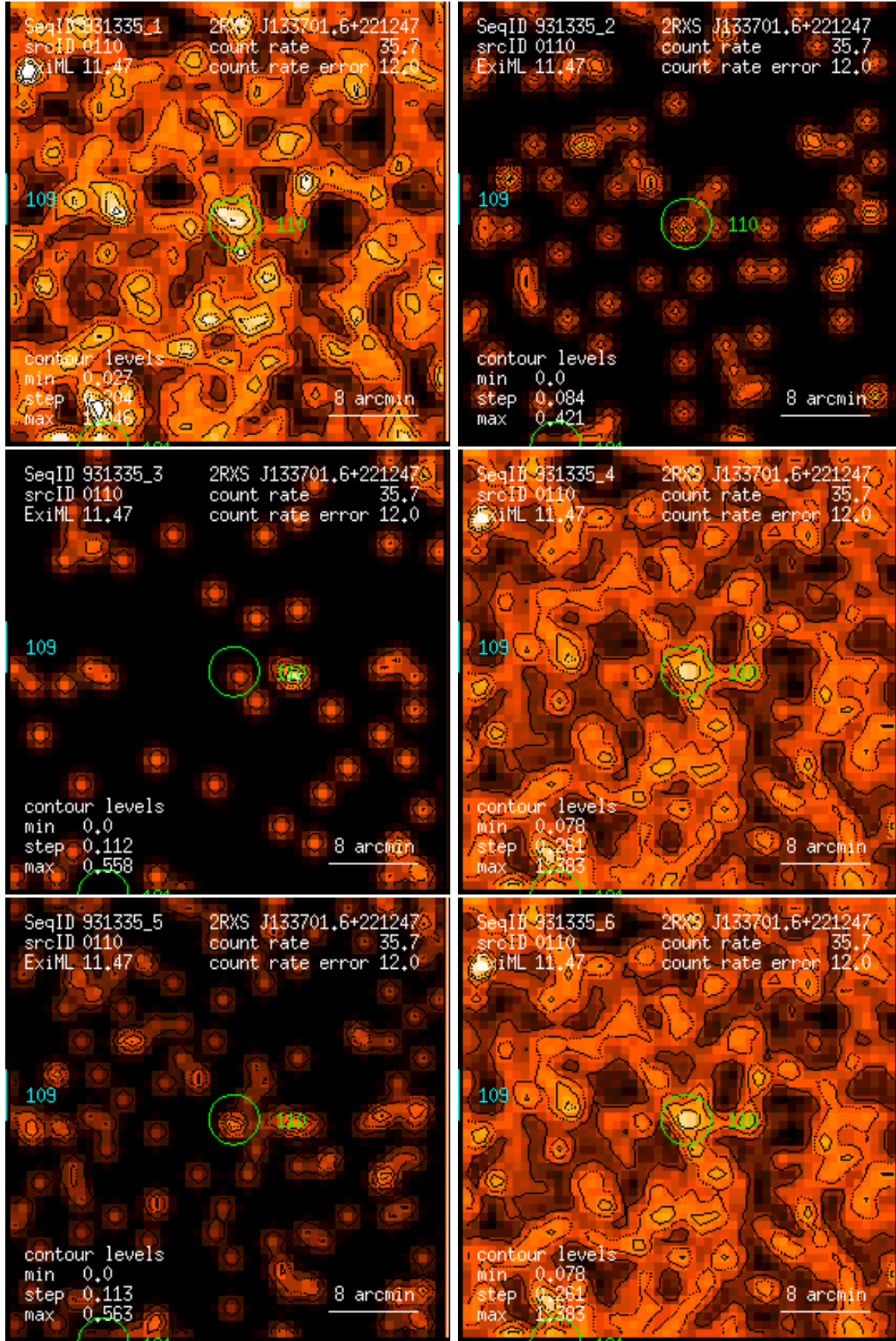
Figure 110: RASS 931335: detection 0110: band rate images, Gaussian filter: (1) PSPC channels 11 – 41, (2) 52 – 90, (3) 91 – 201, (4) 11 – 235, (5) 52 – 201, (6) 11 – 201. Broad band rates in counts/ks. Band rate contour levels in counts/ks/arcmin 2 .
