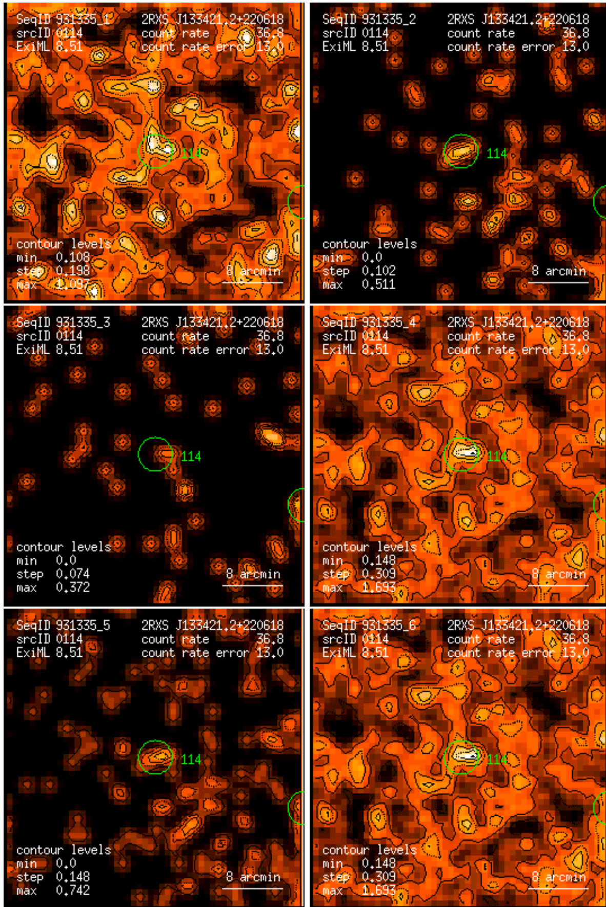
Figure 114: RASS 931335: detection 0114: band rate images, Gaussian filter: (1) PSPC channels 11 – 41, (2) 52 – 90, (3) 91 – 201, (4) 11 – 235, (5) 52 – 201, (6) 11 – 201. Broad band rates in counts/ks. Band rate contour levels in counts/ks/arcmin 2 .
