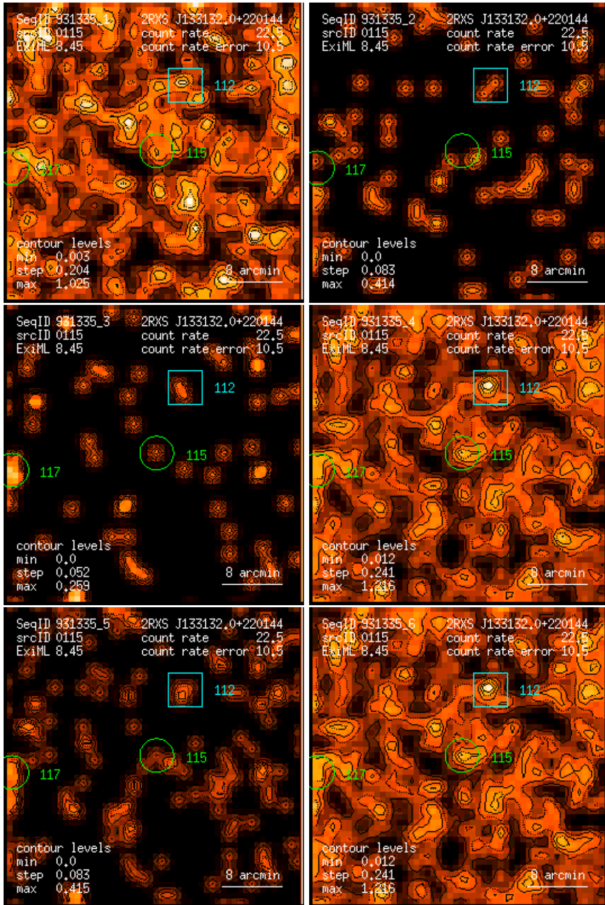
Figure 115: RASS 931335: detection 0115: band rate images, Gaussian filter: (1) PSPC channels 11 – 41, (2) 52 – 90, (3) 91 – 201, (4) 11 – 235, (5) 52 – 201, (6) 11 – 201. Broad band rates in counts/ks. Band rate contour levels in counts/ks/arcmin 2 .
