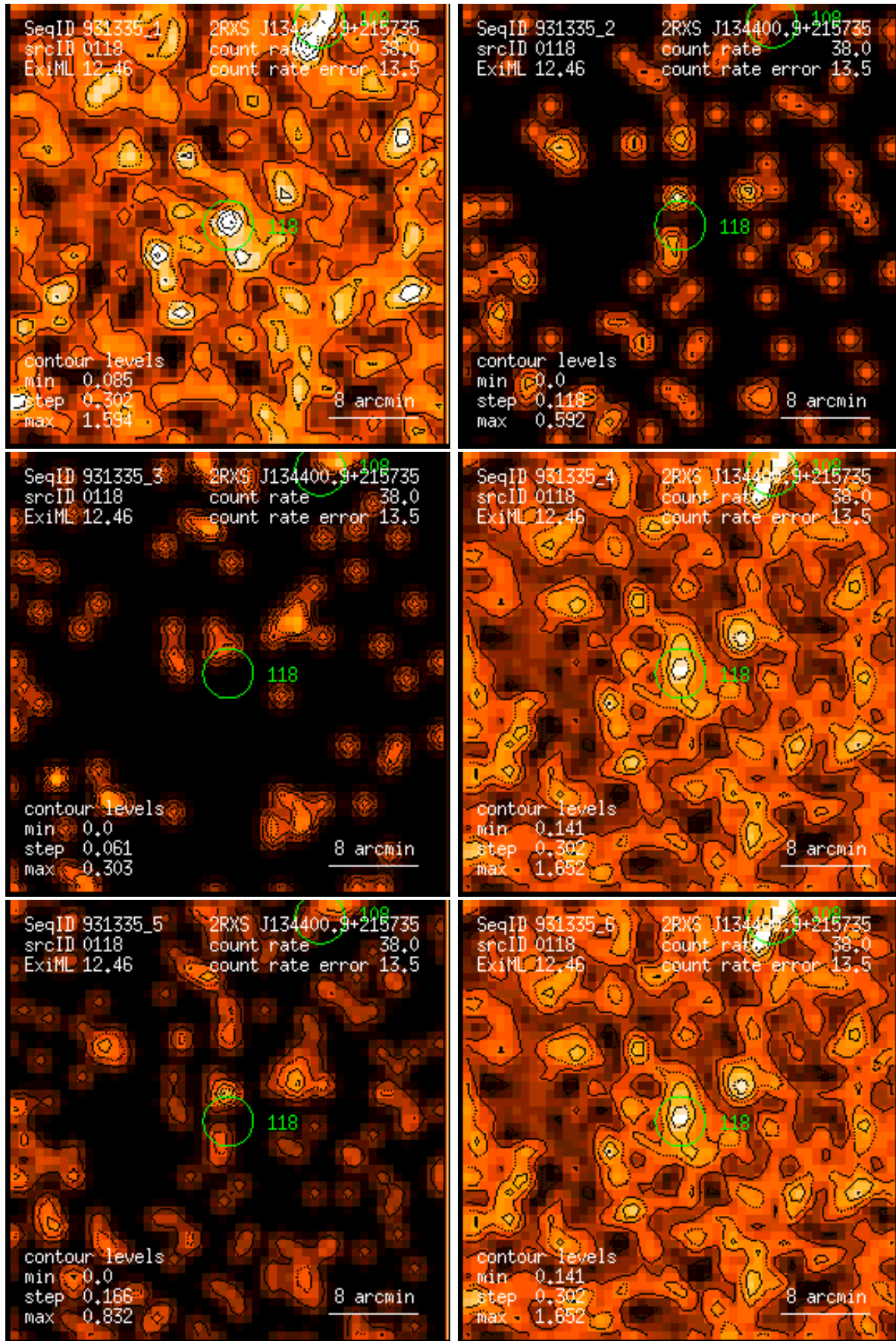
Figure 118: RASS 931335: detection 0118: band rate images, Gaussian filter: (1) PSPC channels 11 – 41, (2) 52 – 90, (3) 91 – 201, (4) 11 – 235, (5) 52 – 201, (6) 11 – 201. Broad band rates in counts/ks. Band rate contour levels in counts/ks/arcmin 2 .
