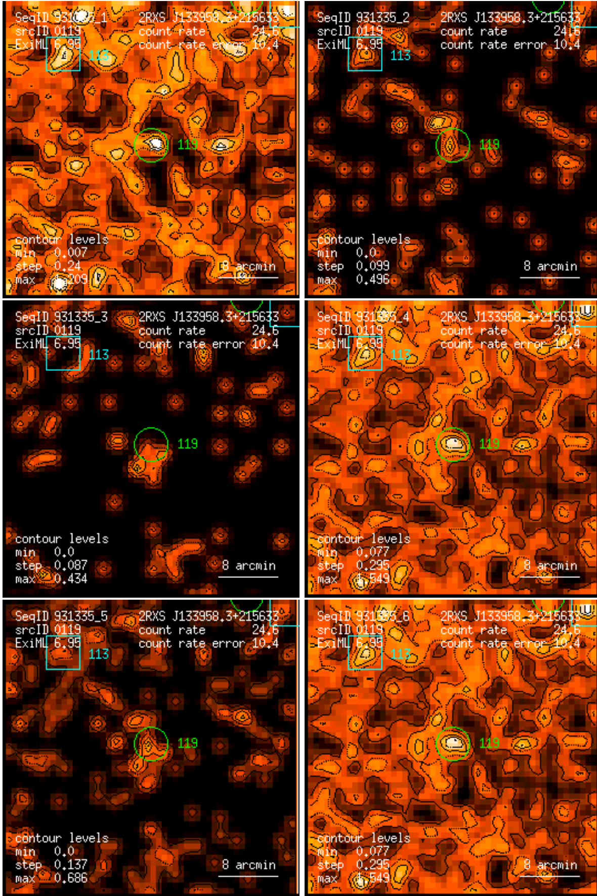
Figure 119: RASS 931335: detection 0119: band rate images, Gaussian filter: (1) PSPC channels 11 – 41, (2) 52 – 90, (3) 91 – 201, (4) 11 – 235, (5) 52 – 201, (6) 11 – 201. Broad band rates in counts/ks. Band rate contour levels in counts/ks/arcmin 2 .
