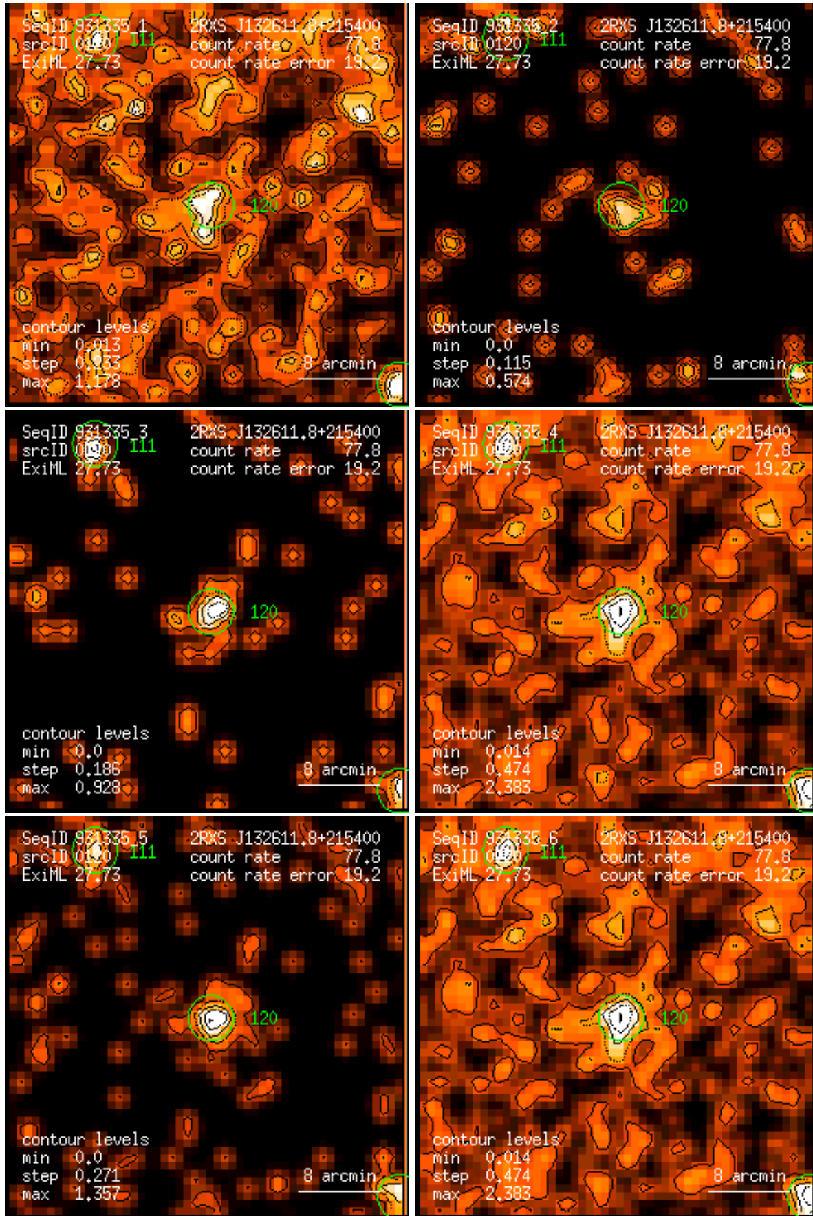
Figure 120: RASS 931335: detection 0120: band rate images, Gaussian filter: (1) PSPC channels 11 – 41, (2) 52 – 90, (3) 91 – 201, (4) 11 – 235, (5) 52 – 201, (6) 11 – 201. Broad band rates in counts/ks. Band rate contour levels in counts/ks/arcmin 2 .
