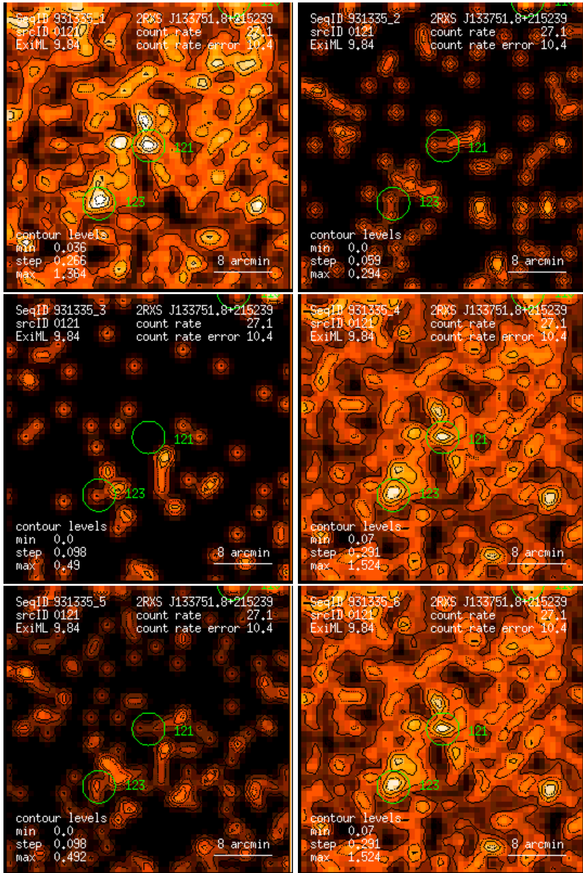
Figure 121: RASS 931335: detection 0121: band rate images, Gaussian filter: (1) PSPC channels 11 – 41, (2) 52 – 90, (3) 91 – 201, (4) 11 – 235, (5) 52 – 201, (6) 11 – 201. Broad band rates in counts/ks. Band rate contour levels in counts/ks/arcmin 2 .
