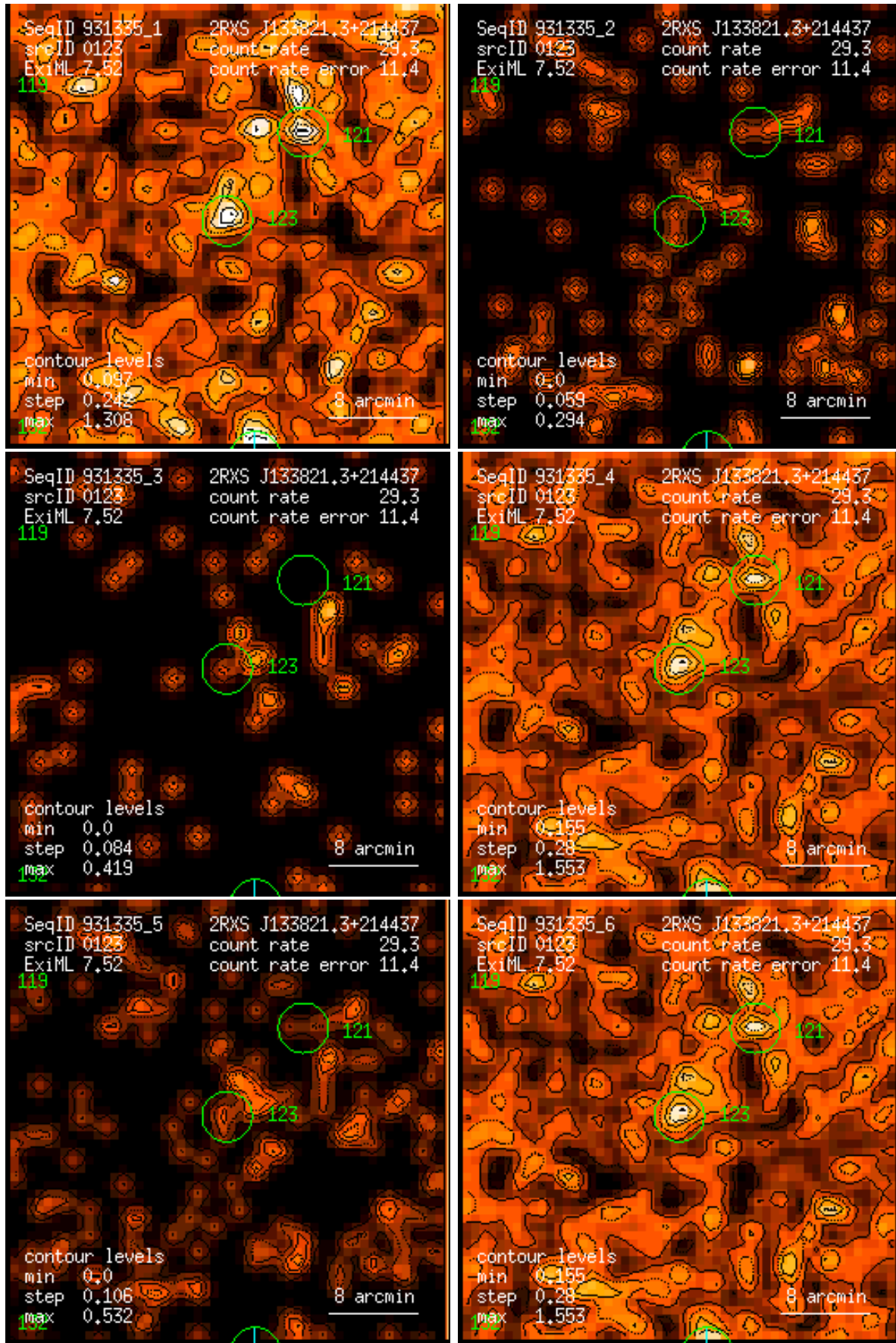
Figure 123: RASS 931335: detection 0123: band rate images, Gaussian filter: (1) PSPC channels 11 – 41, (2) 52 – 90, (3) 91 – 201, (4) 11 – 235, (5) 52 – 201, (6) 11 – 201. Broad band rates in counts/ks. Band rate contour levels in counts/ks/arcmin 2 .
