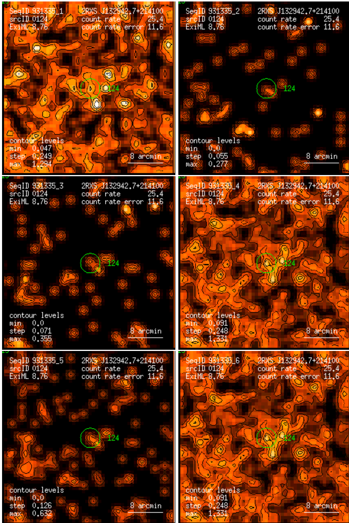
Figure 124: RASS 931335: detection 0124: band rate images, Gaussian filter: (1) PSPC channels 11 – 41, (2) 52 – 90, (3) 91 – 201, (4) 11 – 235, (5) 52 – 201, (6) 11 – 201. Broad band rates in counts/ks. Band rate contour levels in counts/ks/arcmin 2 .
