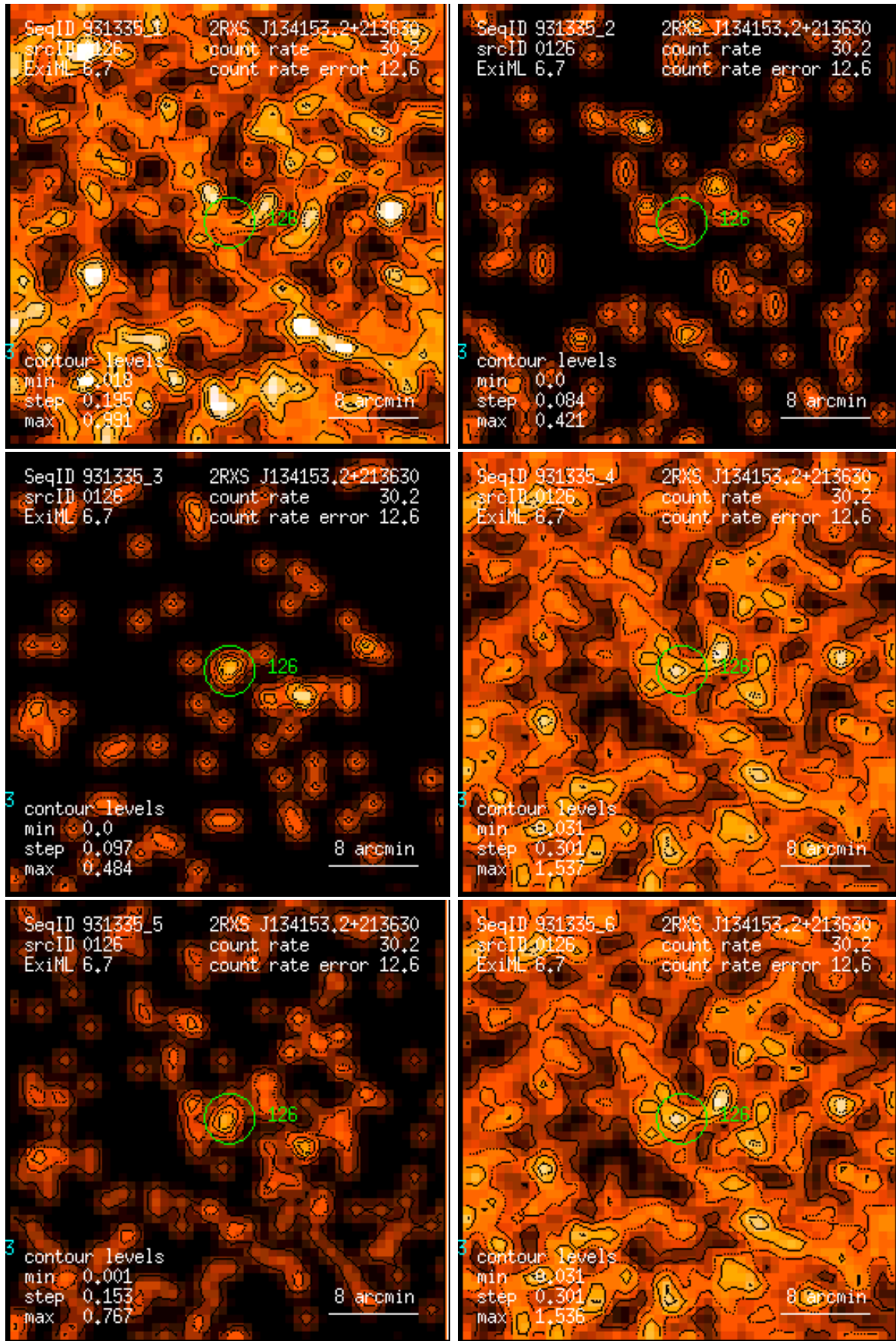
Figure 126: RASS 931335: detection 0126: band rate images, Gaussian filter: (1) PSPC channels 11 – 41, (2) 52 – 90, (3) 91 – 201, (4) 11 – 235, (5) 52 – 201, (6) 11 – 201. Broad band rates in counts/ks. Band rate contour levels in counts/ks/arcmin 2 .
