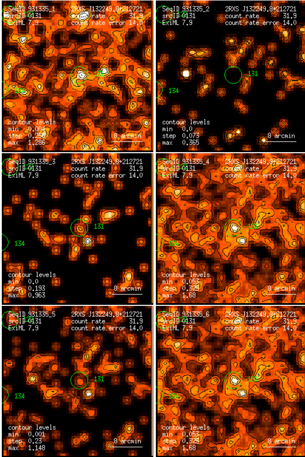
Figure 131: RASS 931335: detection 0131: band rate images, Gaussian filter: (1) PSPC channels 11 – 41, (2) 52 – 90, (3) 91 – 201, (4) 11 – 235, (5) 52 – 201, (6) 11 – 201. Broad band rates in counts/ks. Band rate contour levels in counts/ks/arcmin 2 .
