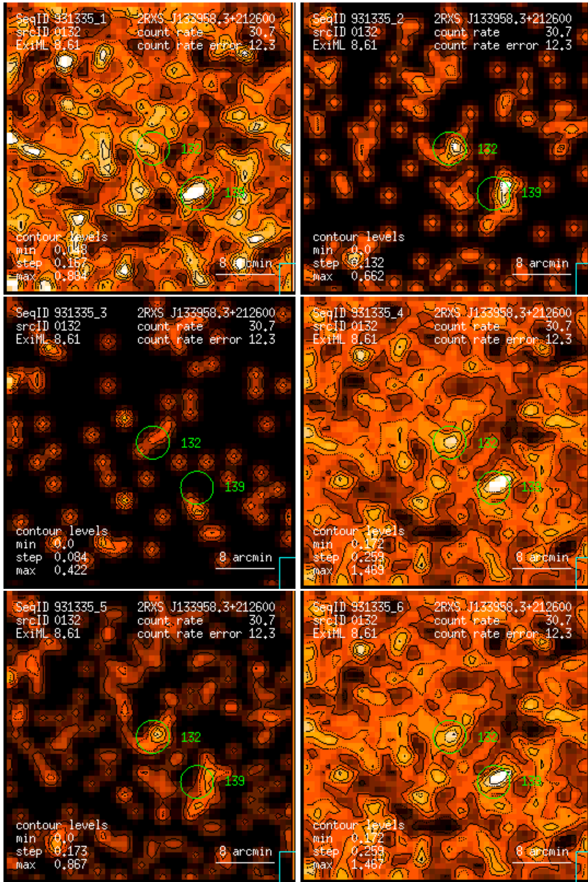
Figure 132: RASS 931335: detection 0132: band rate images, Gaussian filter: (1) PSPC channels 11 – 41, (2) 52 – 90, (3) 91 – 201, (4) 11 – 235, (5) 52 – 201, (6) 11 – 201. Broad band rates in counts/ks. Band rate contour levels in counts/ks/arcmin 2 .
