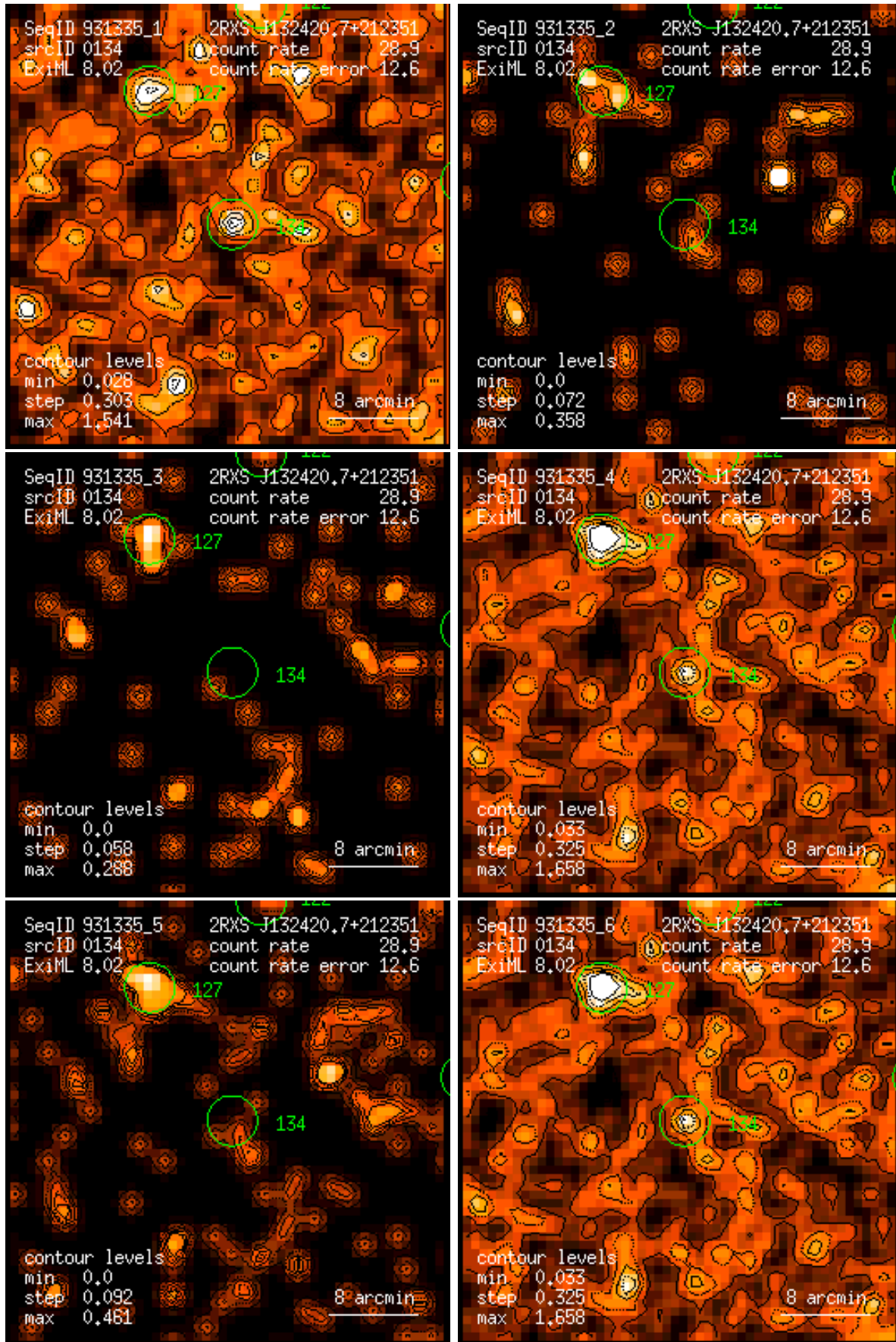
Figure 134: RASS 931335: detection 0134: band rate images, Gaussian filter: (1) PSPC channels 11 – 41, (2) 52 – 90, (3) 91 – 201, (4) 11 – 235, (5) 52 – 201, (6) 11 – 201. Broad band rates in counts/ks. Band rate contour levels in counts/ks/arcmin 2 .
