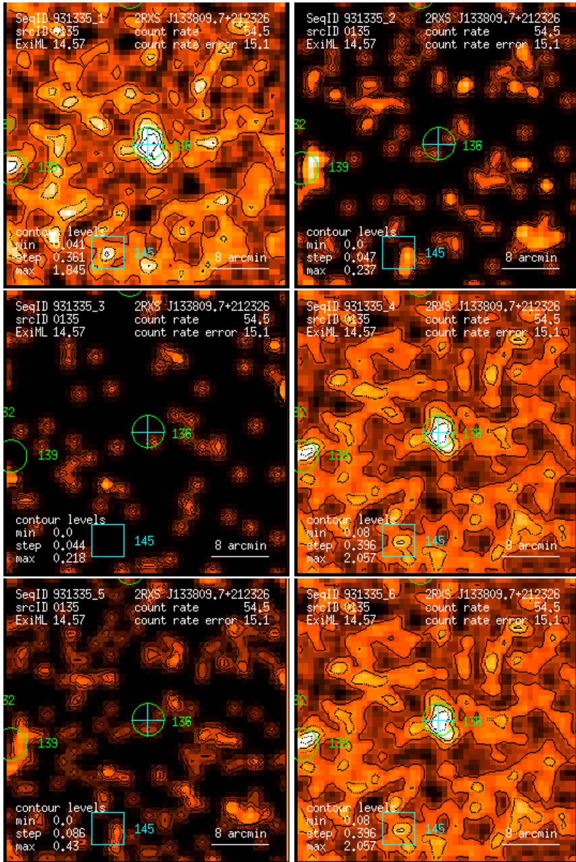
Figure 135: RASS 931335: detection 0135: band rate images, Gaussian filter: (1) PSPC channels 11 – 41, (2) 52 – 90, (3) 91 – 201, (4) 11 – 235, (5) 52 – 201, (6) 11 – 201. Broad band rates in counts/ks. Band rate contour levels in counts/ks/arcmin 2 .
