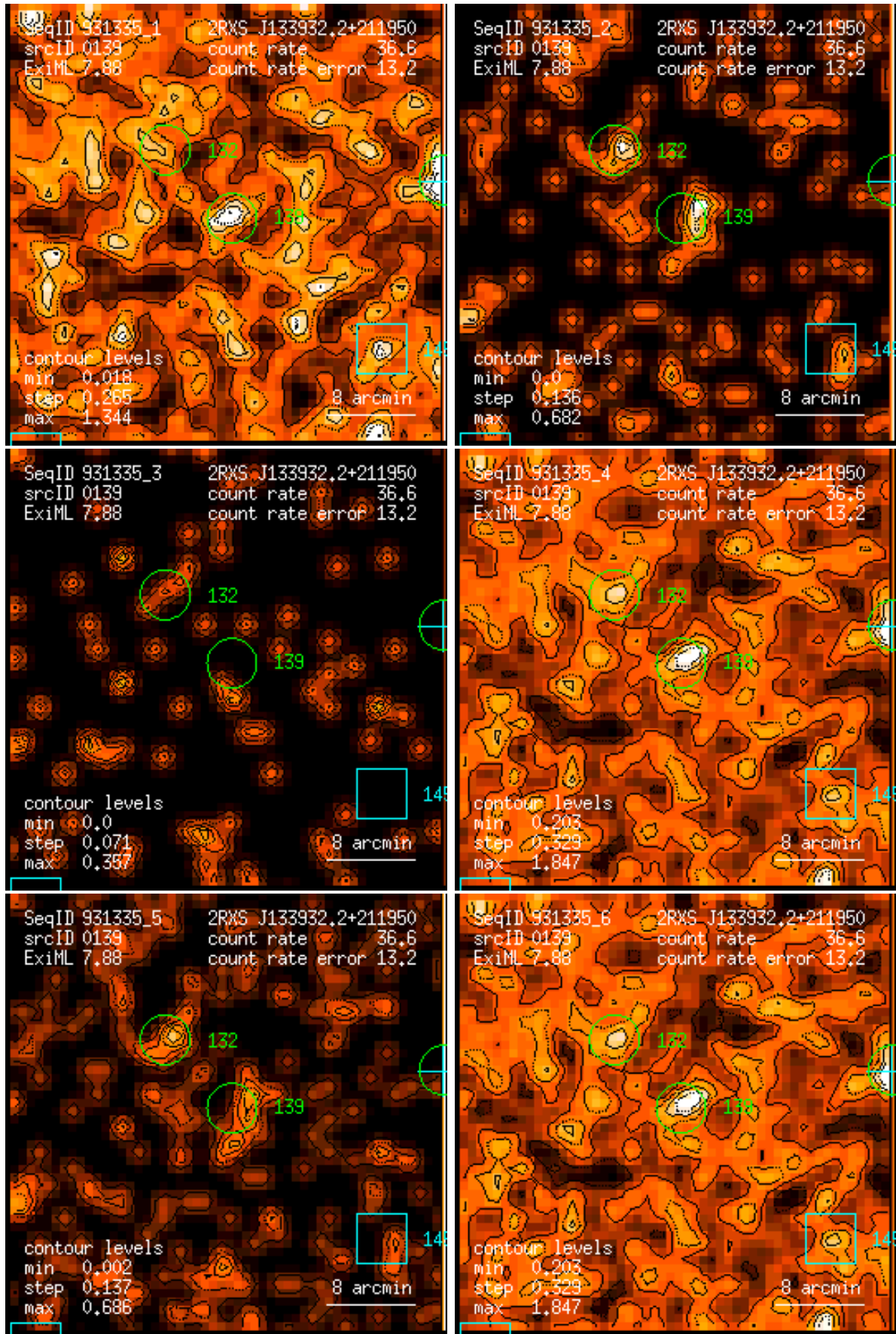
Figure 139: RASS 931335: detection 0139: band rate images, Gaussian filter: (1) PSPC channels 11 – 41, (2) 52 – 90, (3) 91 – 201, (4) 11 – 235, (5) 52 – 201, (6) 11 – 201. Broad band rates in counts/ks. Band rate contour levels in counts/ks/arcmin 2 .
