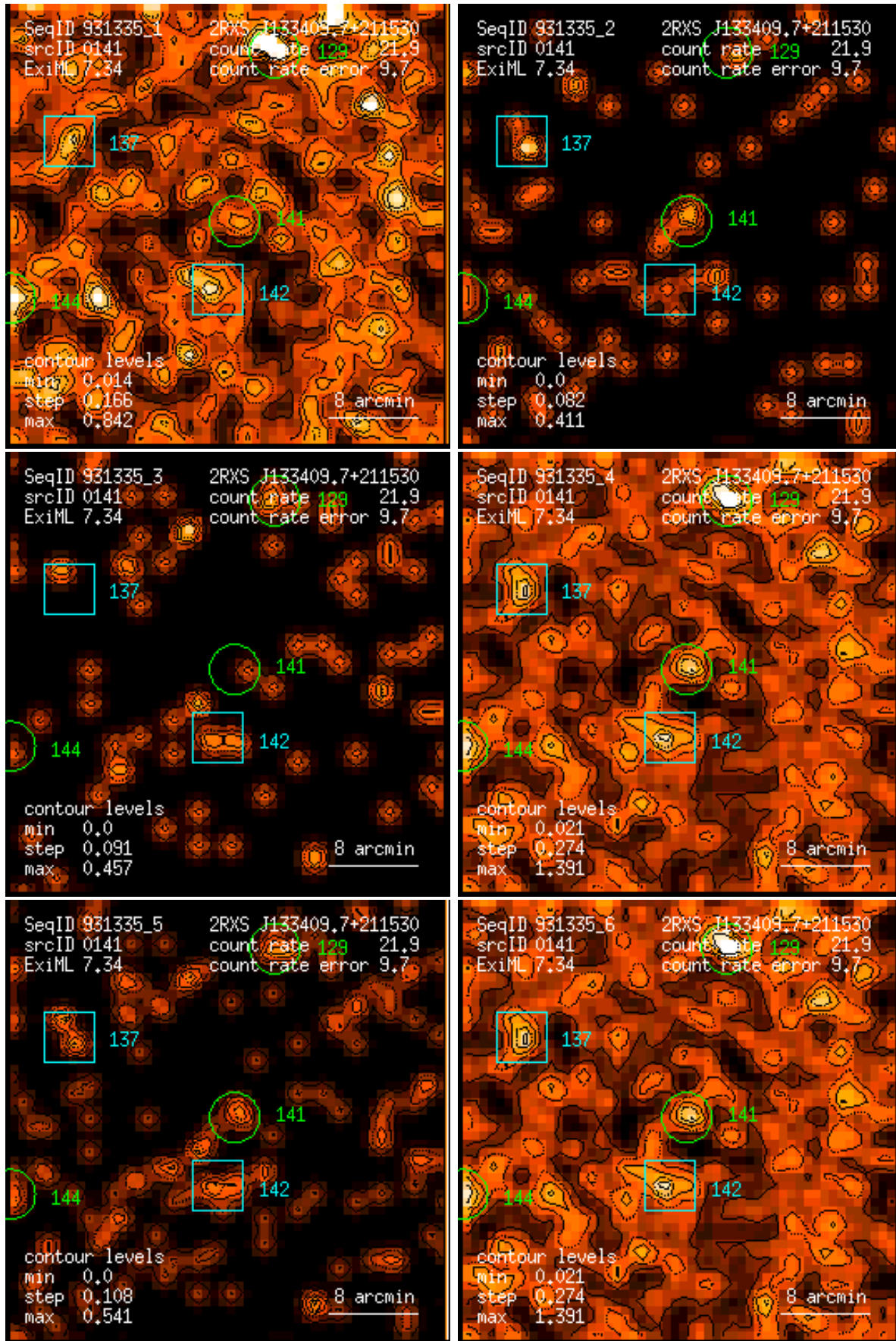
Figure 141: RASS 931335: detection 0141: band rate images, Gaussian filter: (1) PSPC channels 11 – 41, (2) 52 – 90, (3) 91 – 201, (4) 11 – 235, (5) 52 – 201, (6) 11 – 201. Broad band rates in counts/ks. Band rate contour levels in counts/ks/arcmin 2 .
