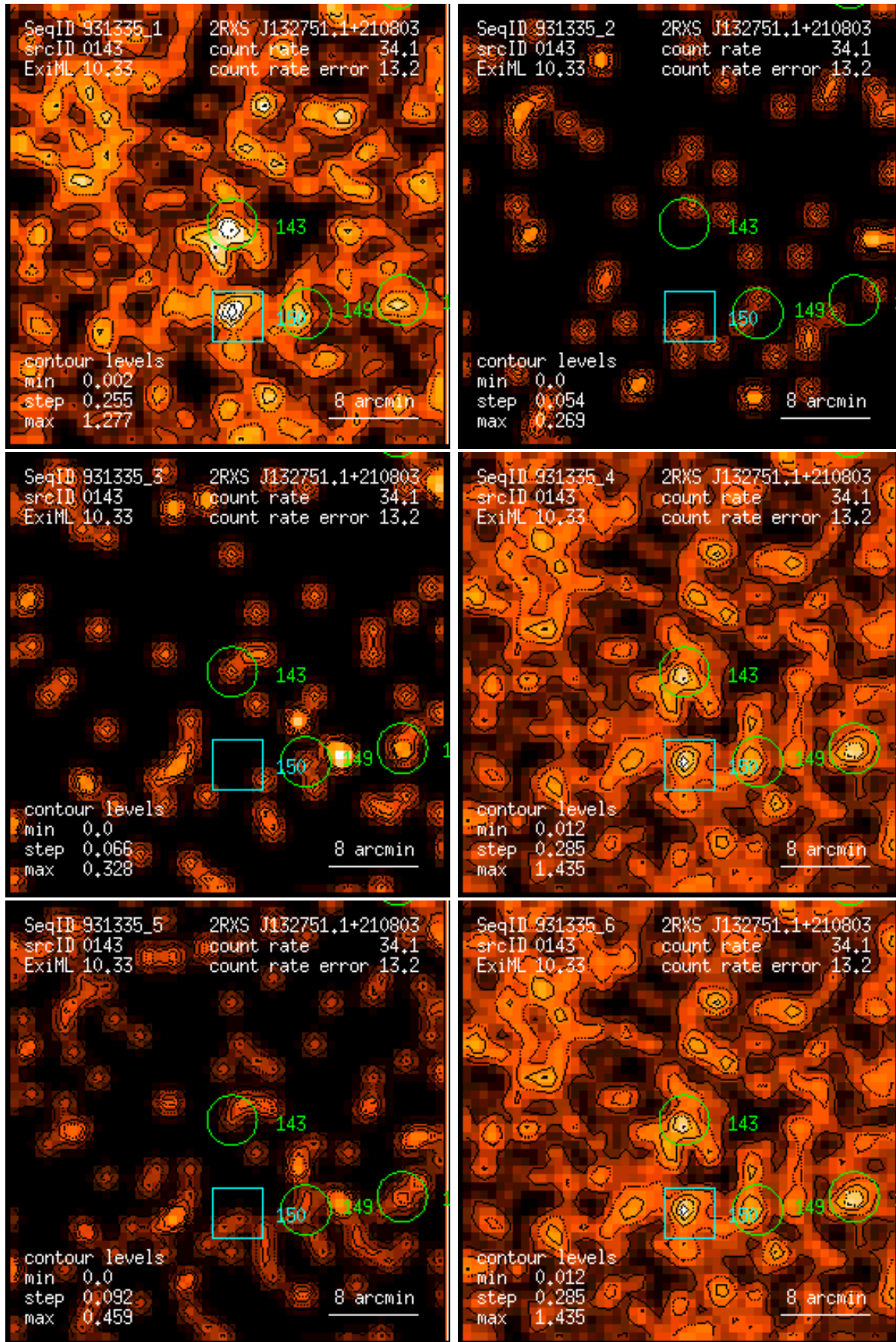
Figure 143: RASS 931335: detection 0143: band rate images, Gaussian filter: (1) PSPC channels 11 – 41, (2) 52 – 90, (3) 91 – 201, (4) 11 – 235, (5) 52 – 201, (6) 11 – 201. Broad band rates in counts/ks. Band rate contour levels in counts/ks/arcmin 2 .
