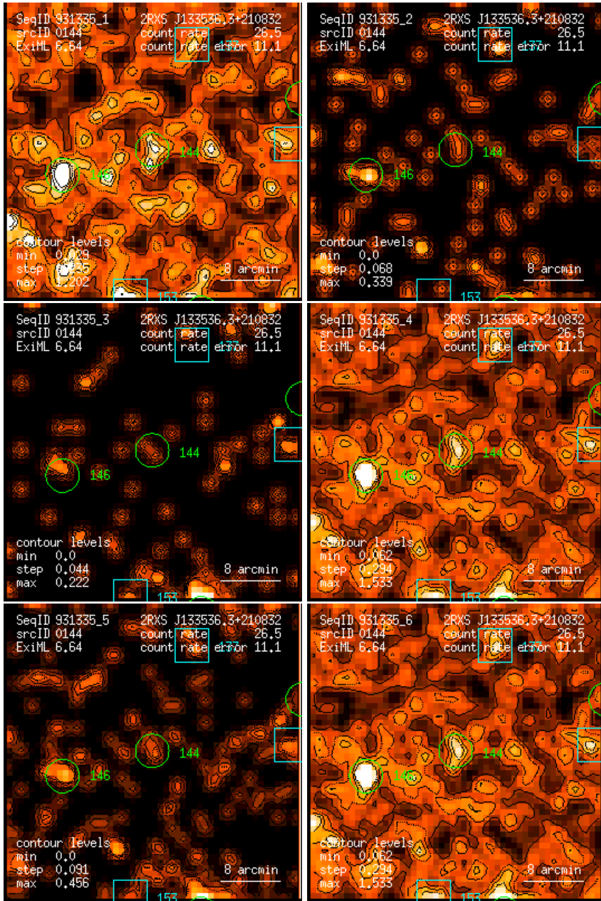
Figure 144: RASS 931335: detection 0144: band rate images, Gaussian filter: (1) PSPC channels 11 – 41, (2) 52 – 90, (3) 91 – 201, (4) 11 – 235, (5) 52 – 201, (6) 11 – 201. Broad band rates in counts/ks. Band rate contour levels in counts/ks/arcmin 2 .
