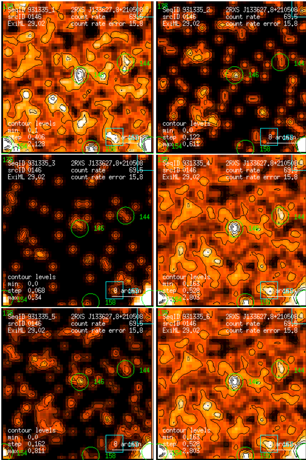
Figure 146: RASS 931335: detection 0146: band rate images, Gaussian filter: (1) PSPC channels 11 – 41, (2) 52 – 90, (3) 91 – 201, (4) 11 – 235, (5) 52 – 201, (6) 11 – 201. Broad band rates in counts/ks. Band rate contour levels in counts/ks/arcmin 2 .
