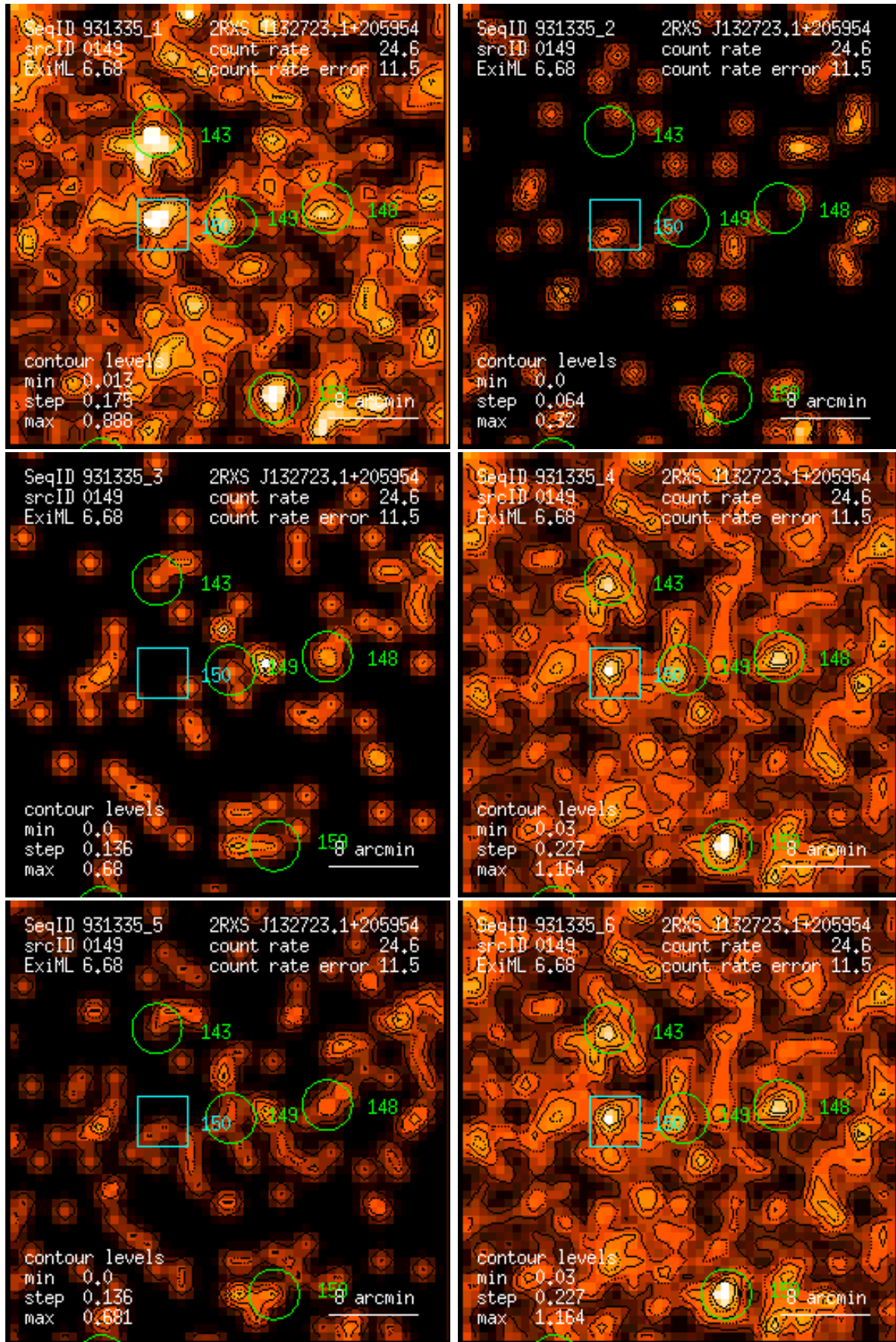
Figure 149: RASS 931335: detection 0149: band rate images, Gaussian filter: (1) PSPC channels 11 – 41, (2) 52 – 90, (3) 91 – 201, (4) 11 – 235, (5) 52 – 201, (6) 11 – 201. Broad band rates in counts/ks. Band rate contour levels in counts/ks/arcmin 2 .
