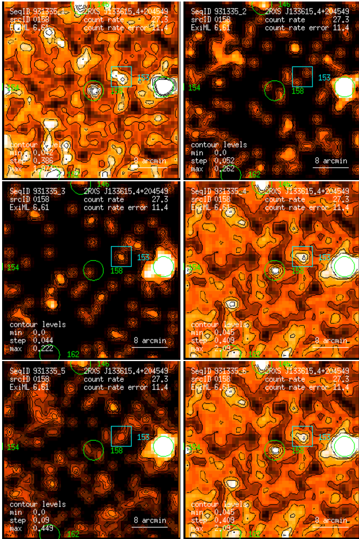
Figure 158: RASS 931335: detection 0158: band rate images, Gaussian filter: (1) PSPC channels 11 – 41, (2) 52 – 90, (3) 91 – 201, (4) 11 – 235, (5) 52 – 201, (6) 11 – 201. Broad band rates in counts/ks. Band rate contour levels in counts/ks/arcmin 2 .
