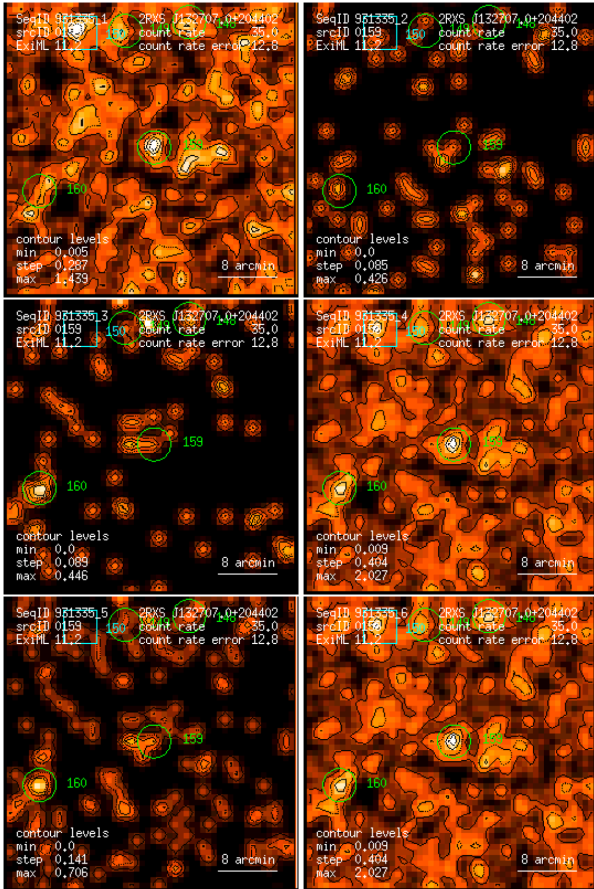
Figure 159: RASS 931335: detection 0159: band rate images, Gaussian filter: (1) PSPC channels 11 – 41, (2) 52 – 90, (3) 91 – 201, (4) 11 – 235, (5) 52 – 201, (6) 11 – 201. Broad band rates in counts/ks. Band rate contour levels in counts/ks/arcmin 2 .
