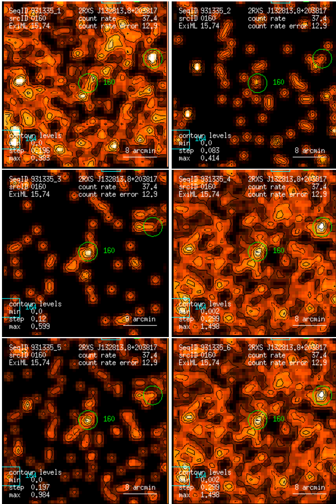
Figure 160: RASS 931335: detection 0160: band rate images, Gaussian filter: (1) PSPC channels 11 – 41, (2) 52 – 90, (3) 91 – 201, (4) 11 – 235, (5) 52 – 201, (6) 11 – 201. Broad band rates in counts/ks. Band rate contour levels in counts/ks/arcmin 2 .
