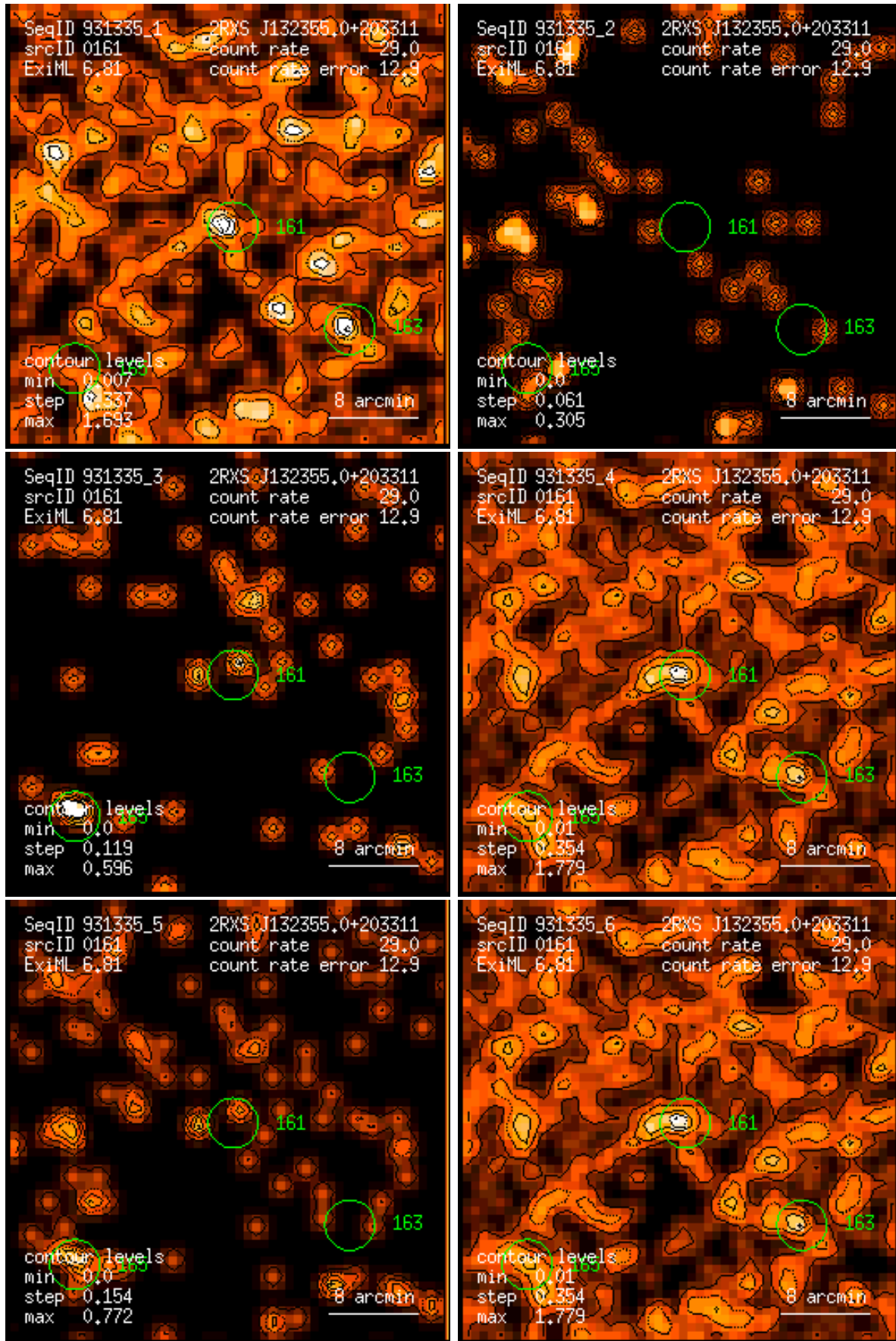
Figure 161: RASS 931335: detection 0161: band rate images, Gaussian filter: (1) PSPC channels 11 – 41, (2) 52 – 90, (3) 91 – 201, (4) 11 – 235, (5) 52 – 201, (6) 11 – 201. Broad band rates in counts/ks. Band rate contour levels in counts/ks/arcmin 2 .
