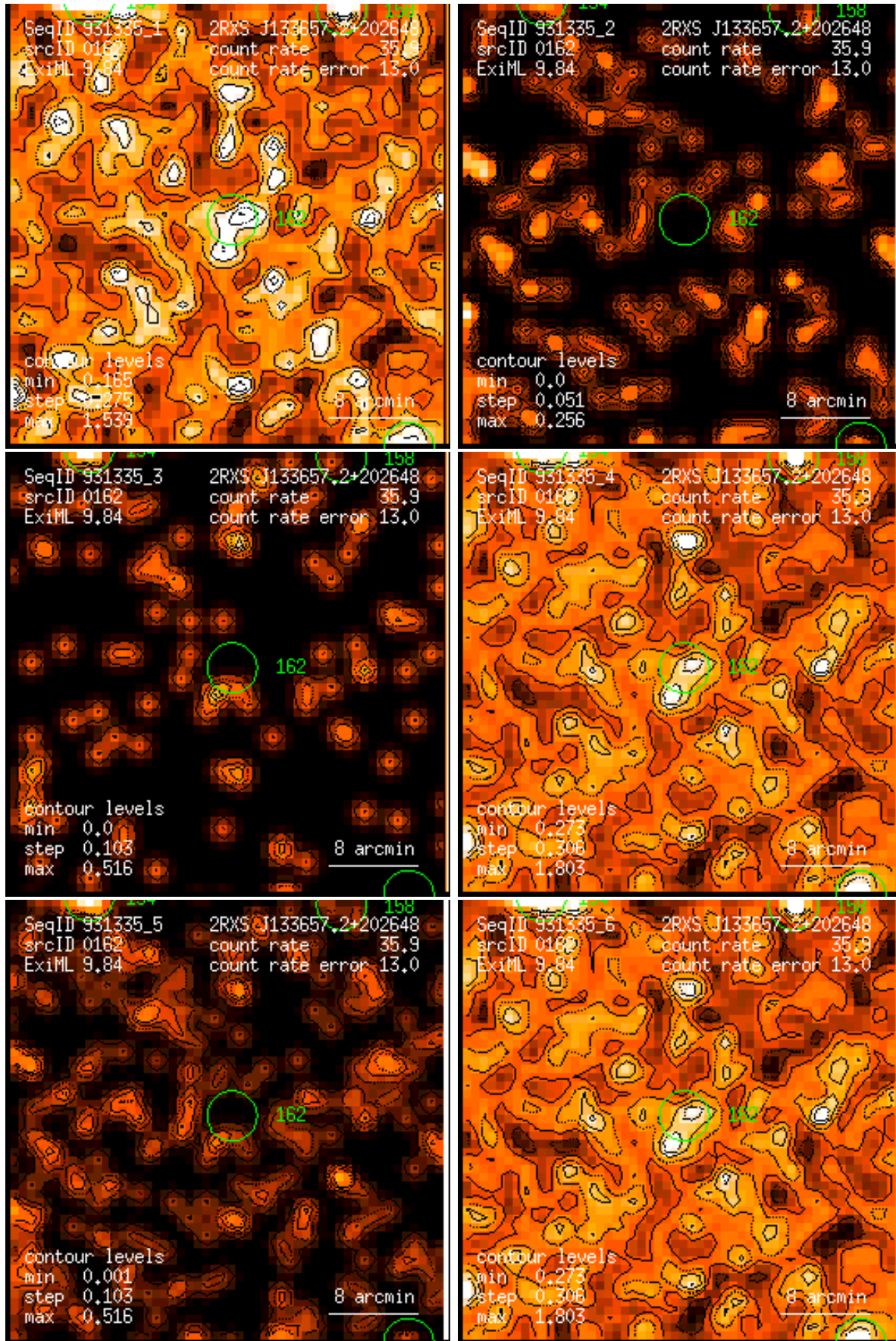
Figure 162: RASS 931335: detection 0162: band rate images, Gaussian filter: (1) PSPC channels 11 – 41, (2) 52 – 90, (3) 91 – 201, (4) 11 – 235, (5) 52 – 201, (6) 11 – 201. Broad band rates in counts/ks. Band rate contour levels in counts/ks/arcmin 2 .
