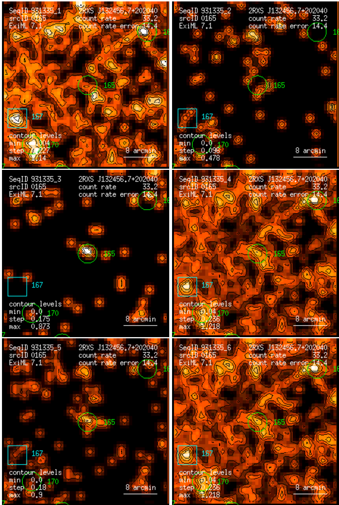
Figure 165: RASS 931335: detection 0165: band rate images, Gaussian filter: (1) PSPC channels 11 – 41, (2) 52 – 90, (3) 91 – 201, (4) 11 – 235, (5) 52 – 201, (6) 11 – 201. Broad band rates in counts/ks. Band rate contour levels in counts/ks/arcmin 2 .
