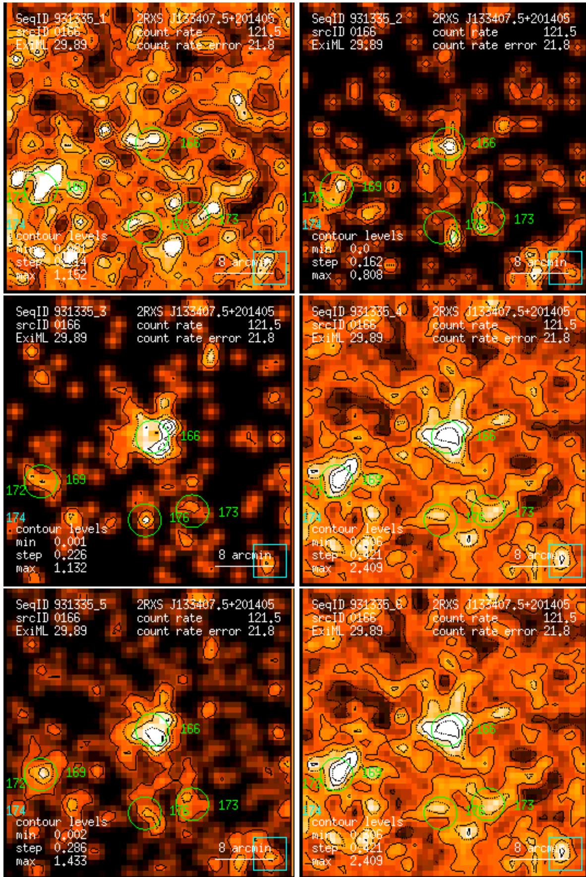
Figure 166: RASS 931335: detection 0166: band rate images, Gaussian filter: (1) PSPC channels 11 – 41, (2) 52 – 90, (3) 91 – 201, (4) 11 – 235, (5) 52 – 201, (6) 11 – 201. Broad band rates in counts/ks. Band rate contour levels in counts/ks/arcmin 2 .
