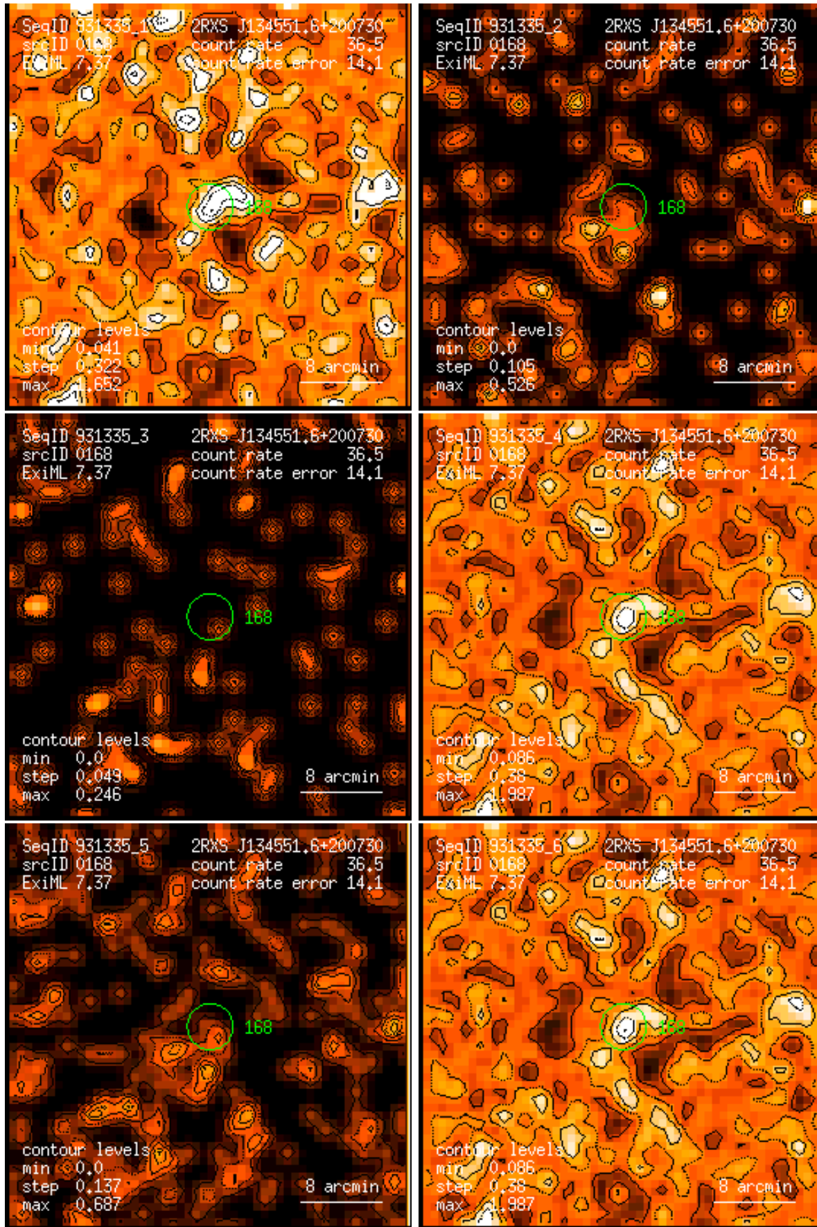
Figure 168: RASS 931335: detection 0168: band rate images, Gaussian filter: (1) PSPC channels 11 – 41, (2) 52 – 90, (3) 91 – 201, (4) 11 – 235, (5) 52 – 201, (6) 11 – 201. Broad band rates in counts/ks. Band rate contour levels in counts/ks/arcmin 2 .
